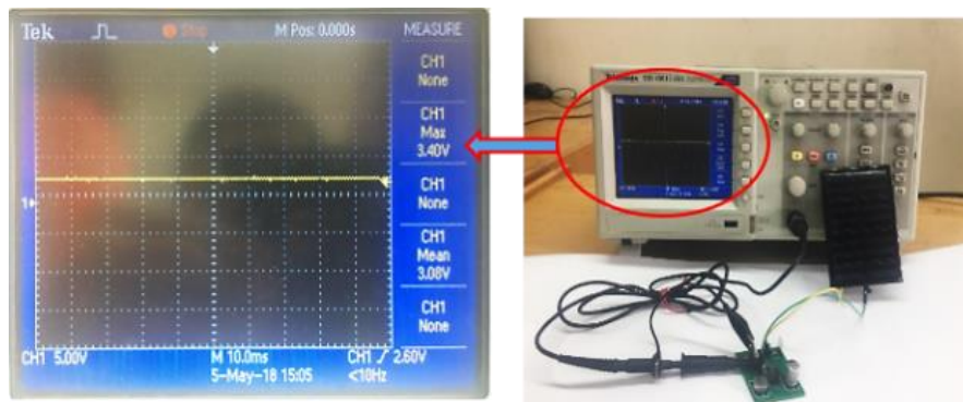
Figure 11. Power supply of WSNN using solar energy harvesting system
