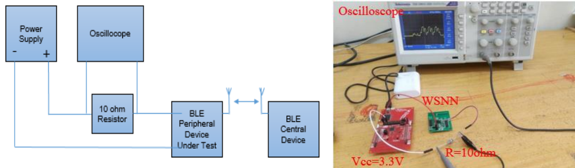
Figure 7. Power consumption measurement setup of the WSNN
