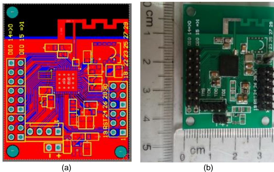
Figure 5. (a) PCB layout of CC2650 integrated MIFA (b) WSNN prototype
