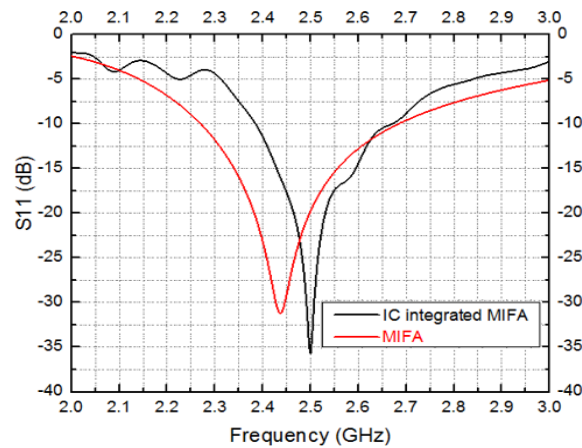
Figure 2. S11 coefficient of MIFA in free-space and model IC integrated MIFA
