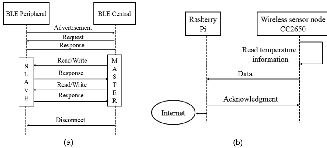
Figure 12. (a) The process of data exchange between two BLE devices (b) The data flow between the WSNN and the Gateway program 6LoWPAN
