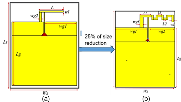
Figure 1. (a) The printed IFA (b) The meander line printed IFA (MIFA)
