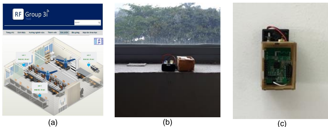
Figure 16. (a) Website interface for indoor temperature monitoring; (b) WSNN installed in the room; (c) Prototype
