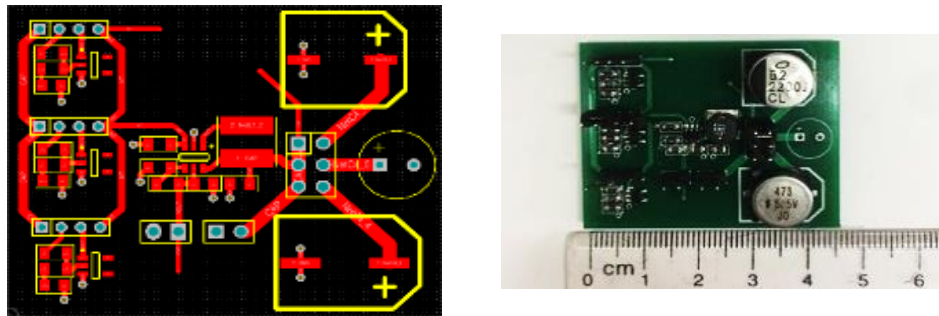
Figure 10. PCB design and prototype of voltage monitor circuit and energy storage
