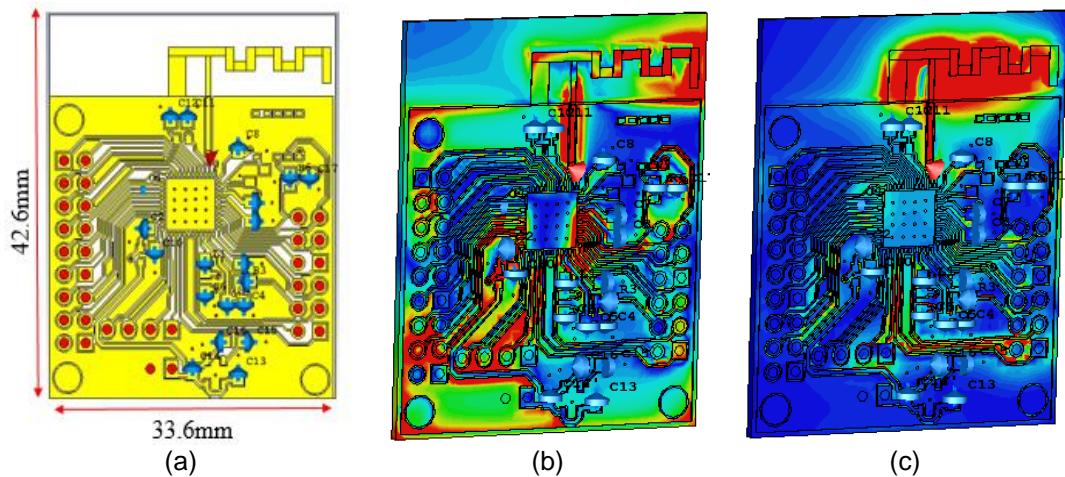
Figure 3. (a) IC integrated MIFA model, (b) E-Field, (c) H-Field
