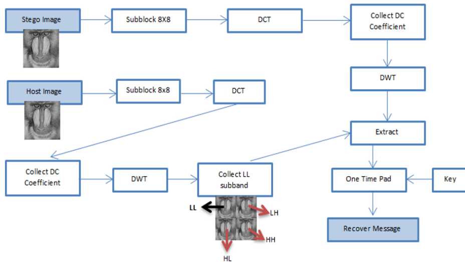
Figure 5. Extraction Scheme using DCT-DWT-OTP
