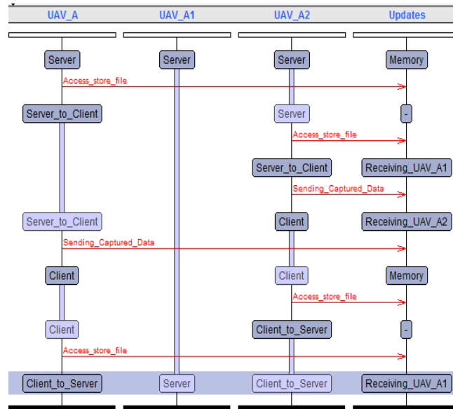
Figure 6. FSRP operation in timed automata
