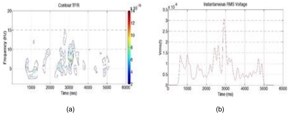
Figure 6. (a) TFR of Gabor transform and (b) V_{rms}(t) plot for window size 300
