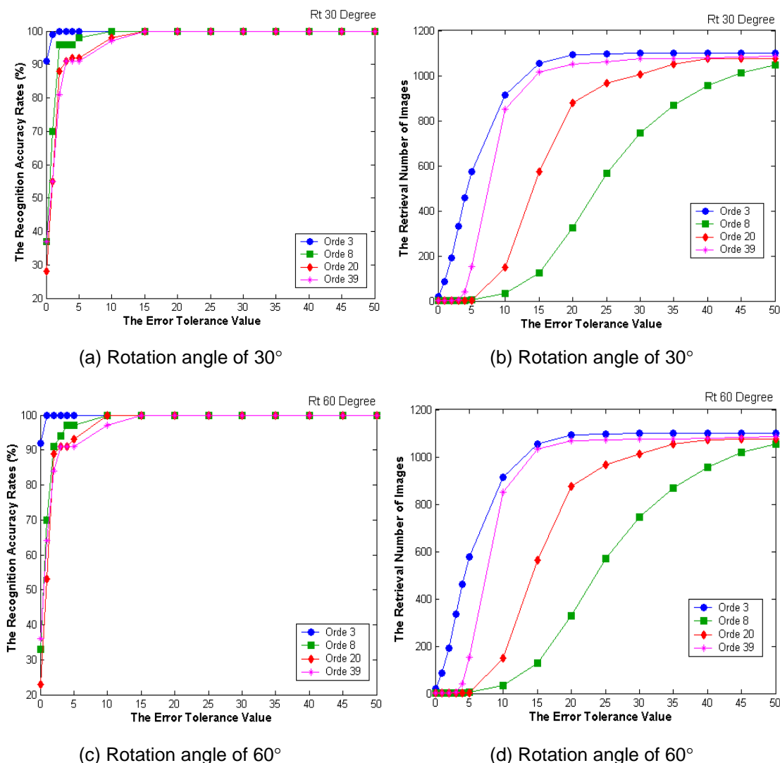
Figure 5. The graphics of the recognition accuracy rates and the retrieval number of images from the image database for rotated query images
