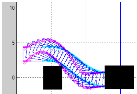
Figure 14. The reversing process on the basis of path planning
