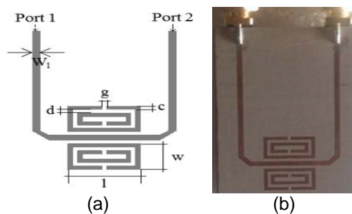
Figure 10. (a) Sensor layout (b) Manufactured prototype [68]
