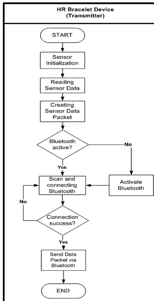
Figure 2. HR sensor transmission flowchart
