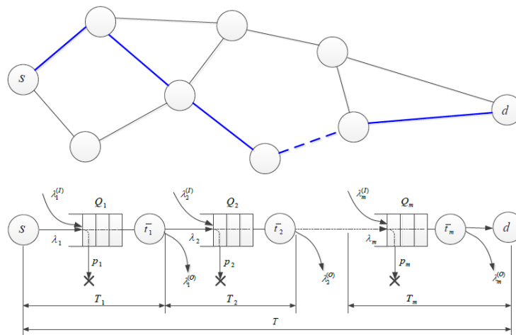
Figure 1. Routing model as a multi-phase queuing system
