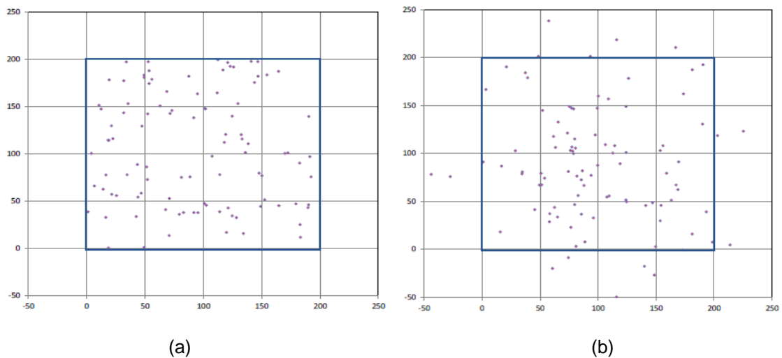
Figure 4. Equipartition (a) and normal (b) laws of distribution of independent coordinates x and y
