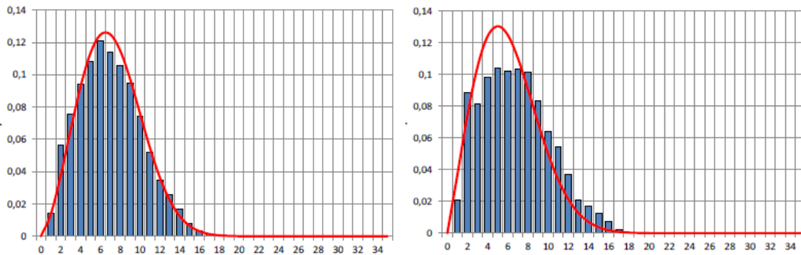
Figure 5. The number of transits in the route for equipartition and normal distribution laws (with equal dispersion)
