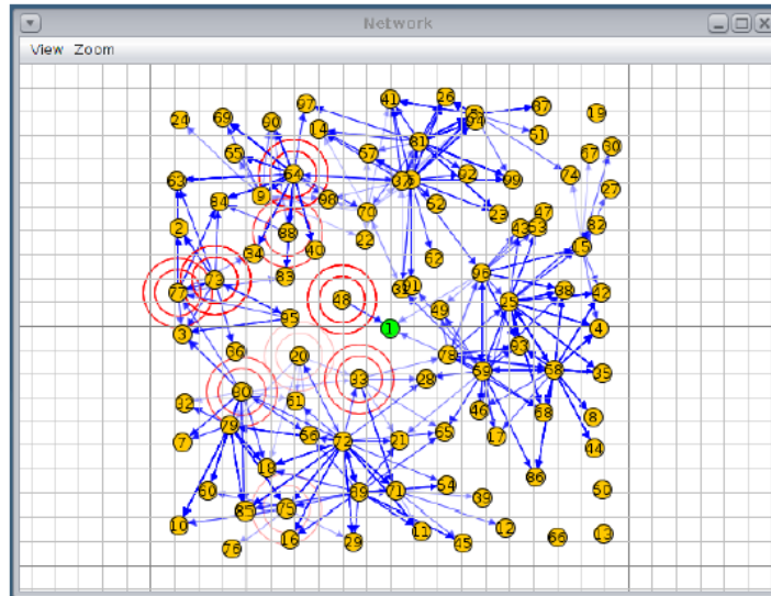
Figure 3. Wireless sensor network model in Contiki simulator (100 nodes, in 200x200 service area)
