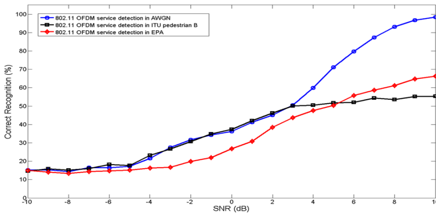
Figure 9. Proposed scheme performance for IEEE 802.11 OFDM service recognition
