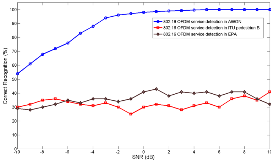
Figure 10. Proposed scheme performance for IEEE 802.16 OFDM service recognition
