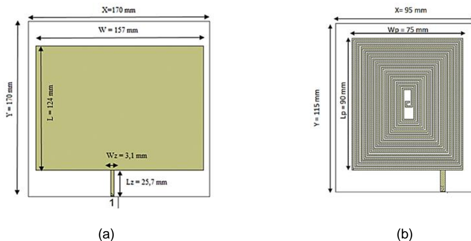
Figure 15. Comparison dimension of conventional microstrip antenna with spiryal labyrinth (a) conventional rectangular patch, (b) spiryal labyrinth patch
