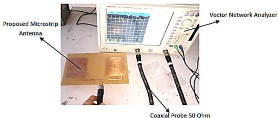
Figure 7. Measurement process of return loss and VSWR
