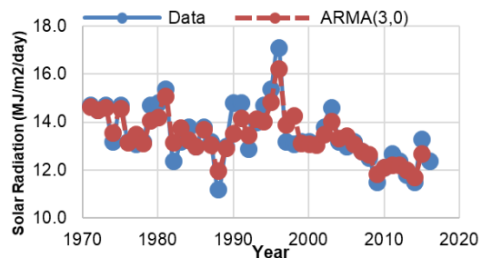
Figure 8. Measured Vs ARMA(3,0) of mean yearly minimum solar radiation (1971-2016)
