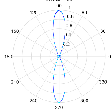
Number of element=7. The pattern multiplication method is shown using blue line and CST is shown in cyan line.
