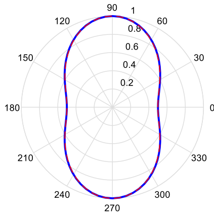
Number of element=2. The pattern multiplication method is shown using blue line and CST is shown in red line.
