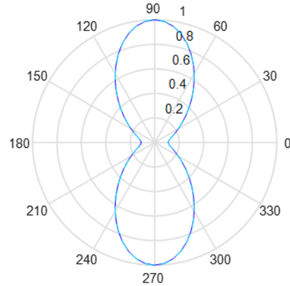
Number of element=3. The pattern multiplication method is shown using blue line and CST is shown in cyan line.
