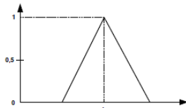
Gambar 5. T-function
