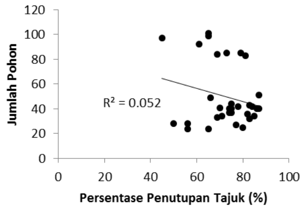
Gambar 3. Hubungan antara peubah persentase penutupan tajuk (C) dan jumlah pohon (N) Figure 3. Relationship between variables percentage canopy cover (C) and number of trees (N)
