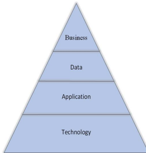
Fig. 1. Enterprise Architecture
