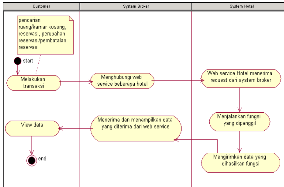
Gambar 4. Activity Diagram
