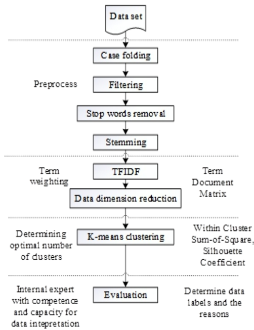
Figure 1. Clustering flow
