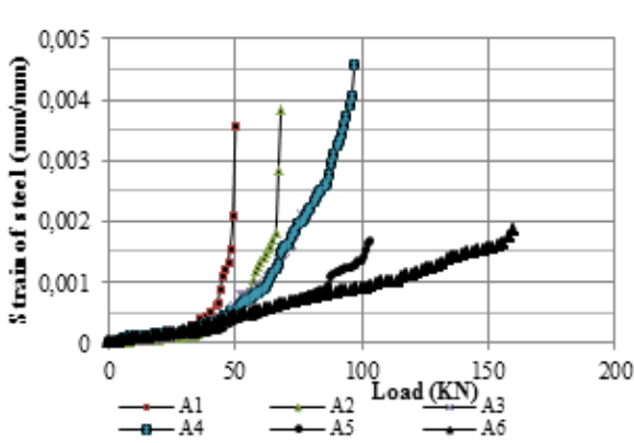
Figure 5. Variation of deflection with load for six types of reinforcement
