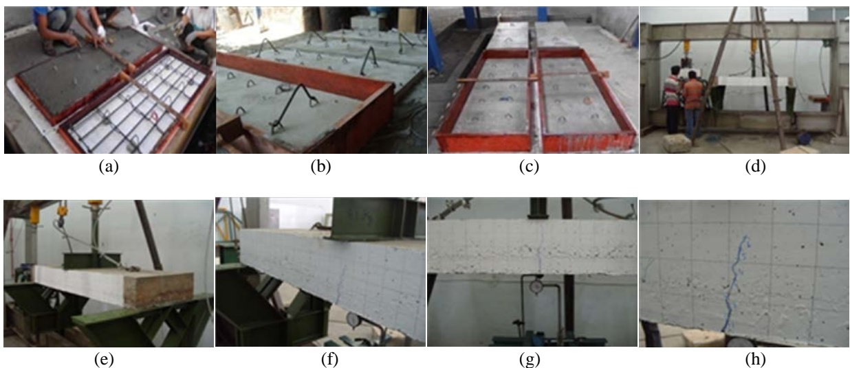
Figure 2. Flexural test specimens
