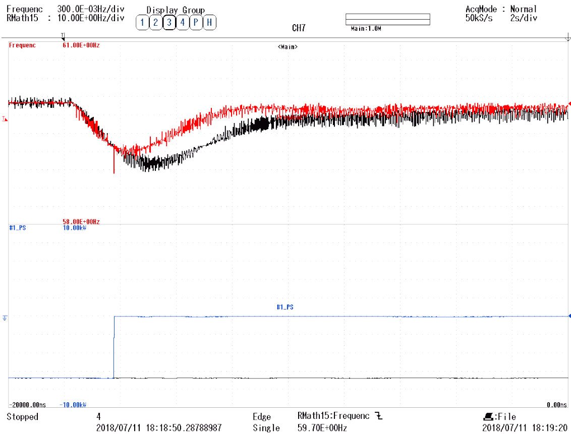
Figure 5.22: Comparison between test with no intervention (in black) and test test with UFLS emulation (in colors). The upper window shows the equipment's output line voltages' frequency. The lower window shows the measured three-phase active power going into Converter 2 .
