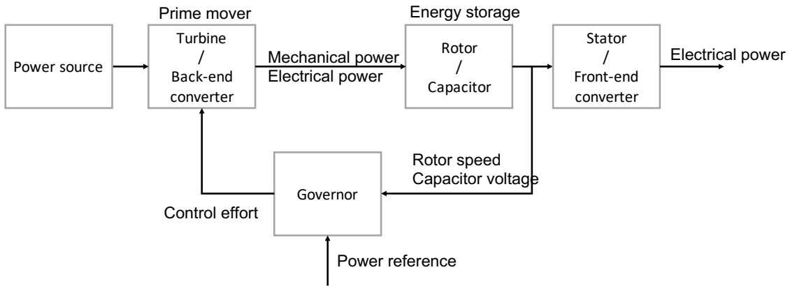
Figure 3.13: Relationship between SSM and SM generating units.
