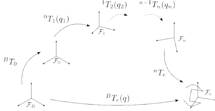
Figure 2.5: Forward kinematics in an open-chain manipulator
