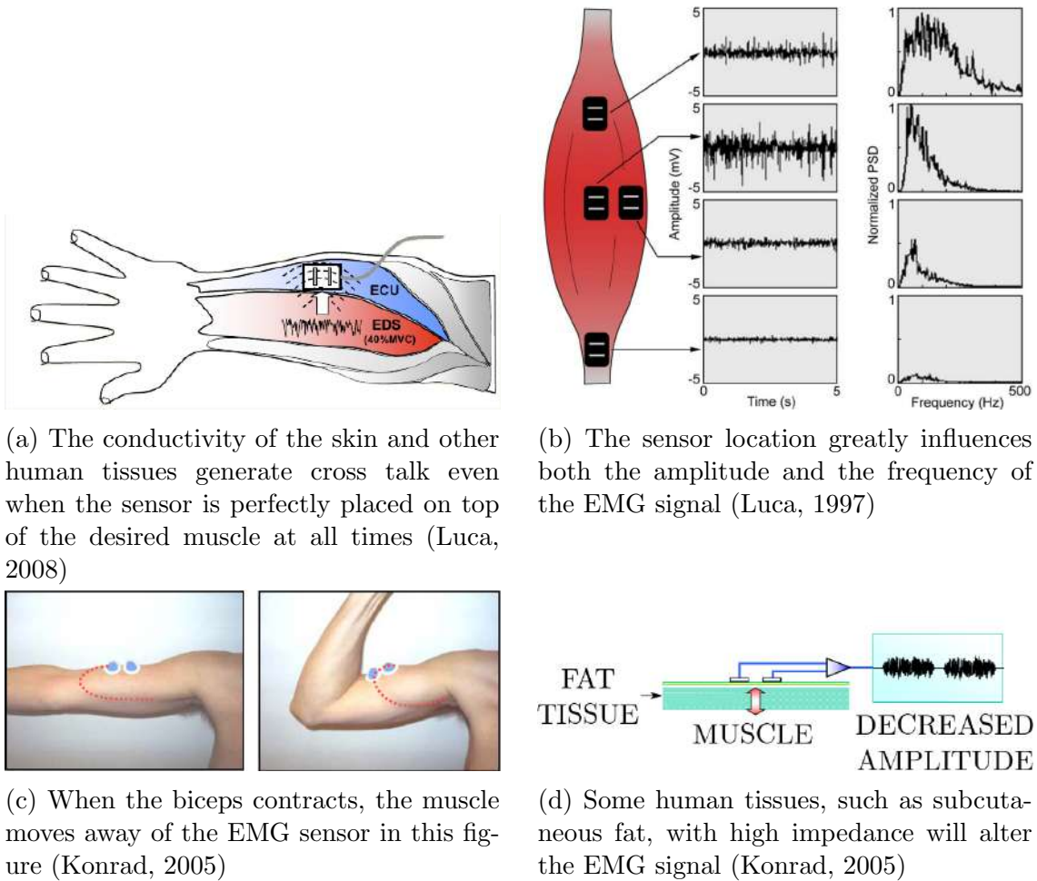
Figure 3.2: Difficulties that arise when acquiring EMG signal
