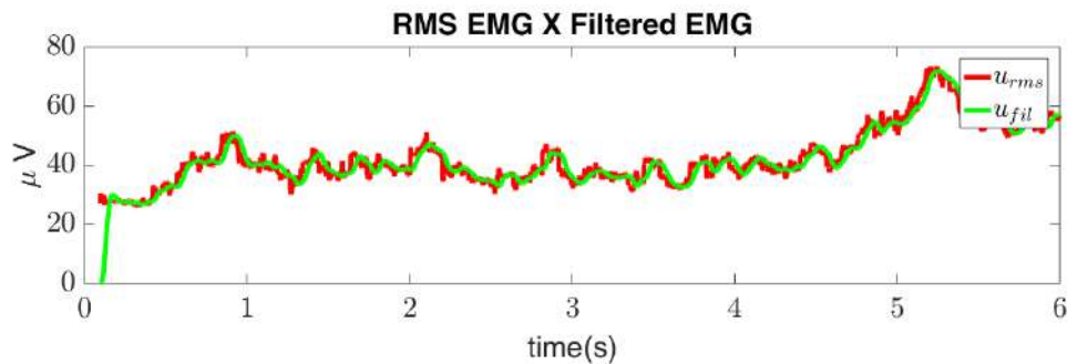
Figure 3.4: Steps to obtain an enveloped EMG signal for this work
