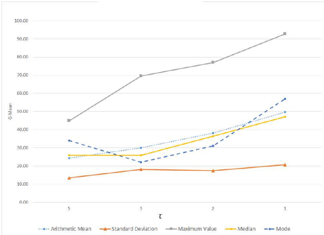
Figure 41 – G-Mean statistics for all stock symbols and time offsets of \tau=1, 2, 3, and 5.
