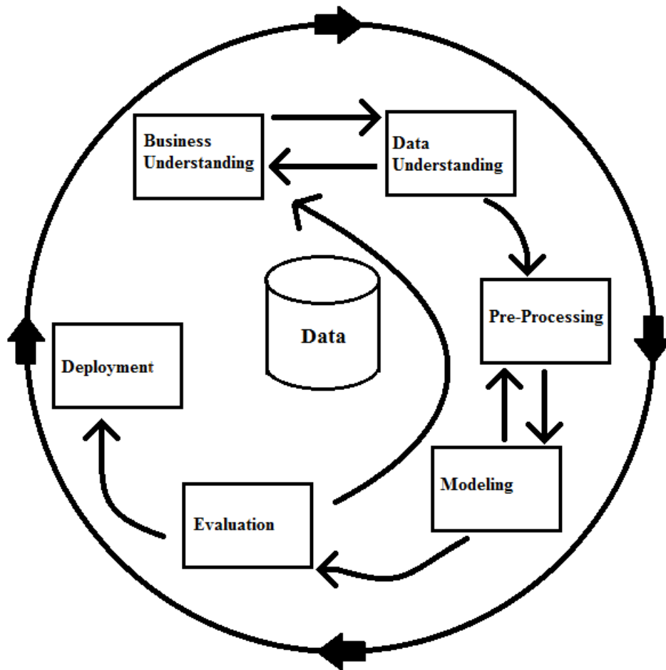
Figure 3 - The CRISP-DM process.
