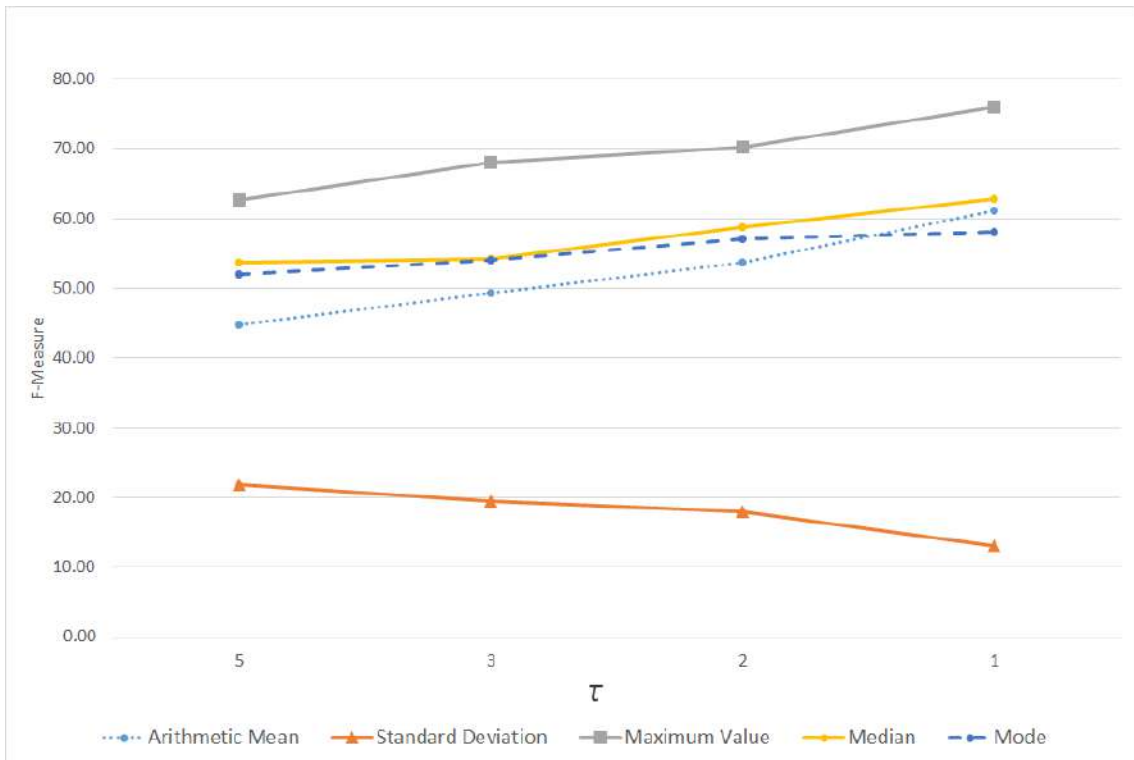
Figure 42 - F-Measure statistics for all stock symbols and time offsets of \tau=1, 2, 3, and 5.
