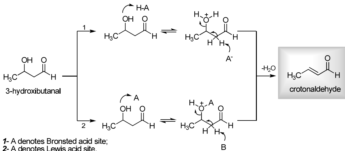
Figure 1.3.4 – Suggested mechanism for crotonaldehyde formation from 3-hydroxibutanal dehydration, involving Brønsted and Lewis acid sites (KALSI, 2006).
