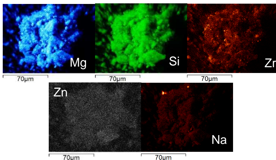
Figure 4.4.10 - Elemental mapping of the 2-Na/ZrZn/MgO-SiO 2 -(50:50) catalyst.
