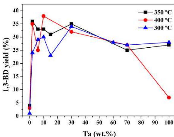
Figure 1.2.4 – Effect of tantalum content of the Ta_2O_5/SiO_2 catalyst and on 1,3-BD yield. Reaction conditions: liquid hourly space velocity of 0.4\ h^{-1} , EtOH/AcH feed ratio of 2.75, atmospheric pressure and TOS = 8 h (CORSON et al. , 1949).
