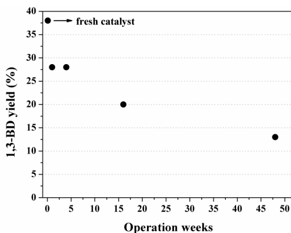
Figure 1.2.3 – Effect of consecutive operation and regeneration cycles on 1,3-BD yield over the Ta_2O_5/SiO_2 catalyst. Reaction conditions: 350 °C, liquid hourly space velocity of 0.4\ h^{-1} , EtOH/AcH feed ratio of 2.75 and atmospheric pressure (CORSON et al. , 1949).
