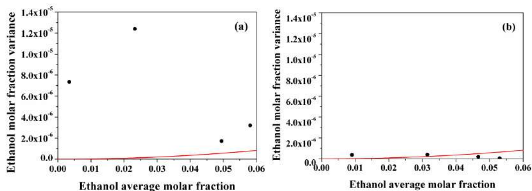
Figure 4.2.7 – Variances of ethanol molar fractions for catalytic reactions (●) and chromatographic measurement fluctuation model (-) as functions of ethanol average molar fractions for catalysts MgO-SiO 2 -(50:50) (a) and MgO-SiO 2 -(95:5) (b).
