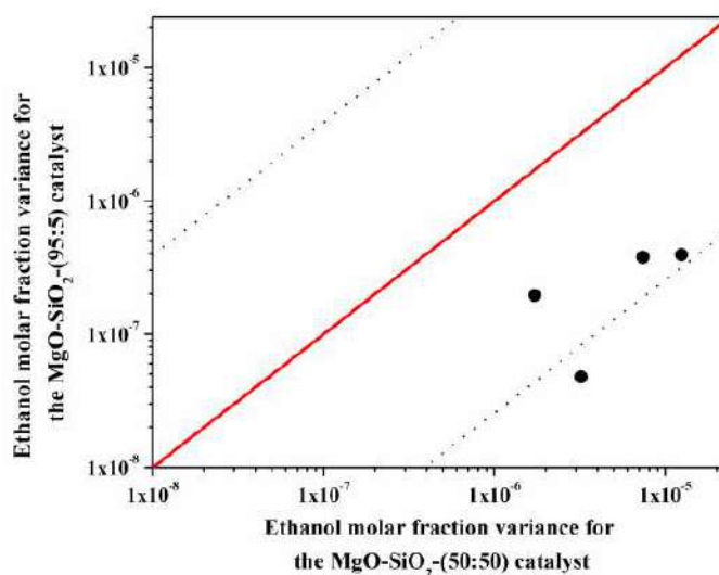
Figure 4.2.13 – Variances of ethanol molar fractions for catalysts MgO-SiO 2 -(50:50) and MgO-SiO 2 -(95:5).
