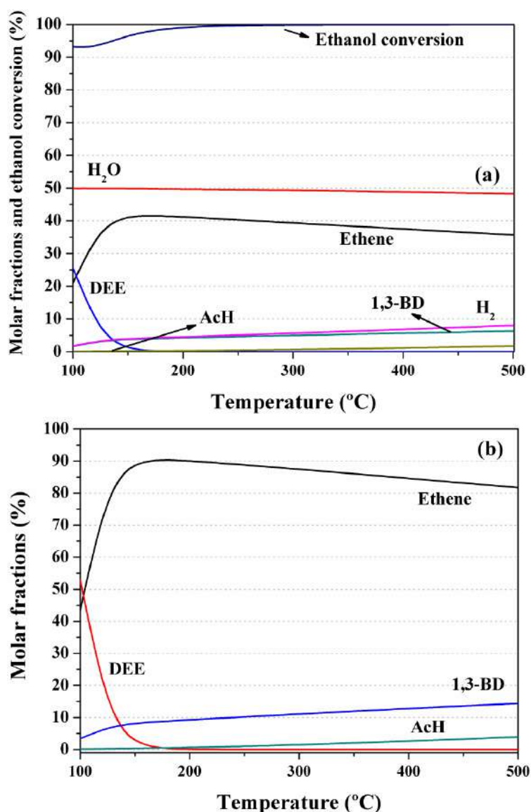
Figure 1.4.3 – Equilibrium composition at 1 atm, using pure ethanol as reactant (2 mols). The following compounds were allowed to be present at the equilibrium: ethanol, ethene, DEE, H 2 O, AcH, H 2 and 1,3-BD. In (a), molar fractions were calculated excluding ethanol; in (b), molar fractions were calculated excluding ethanol, water and hydrogen.
