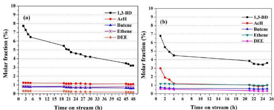
Figure 4.5.4 - Effect of time on stream on the molar fraction of the main carbon containing products: (a) fresh catalyst; (b) recycled catalyst. (T of 350 °C, WHSV of 0.62 h -1 , contact time of 3.8 s).
