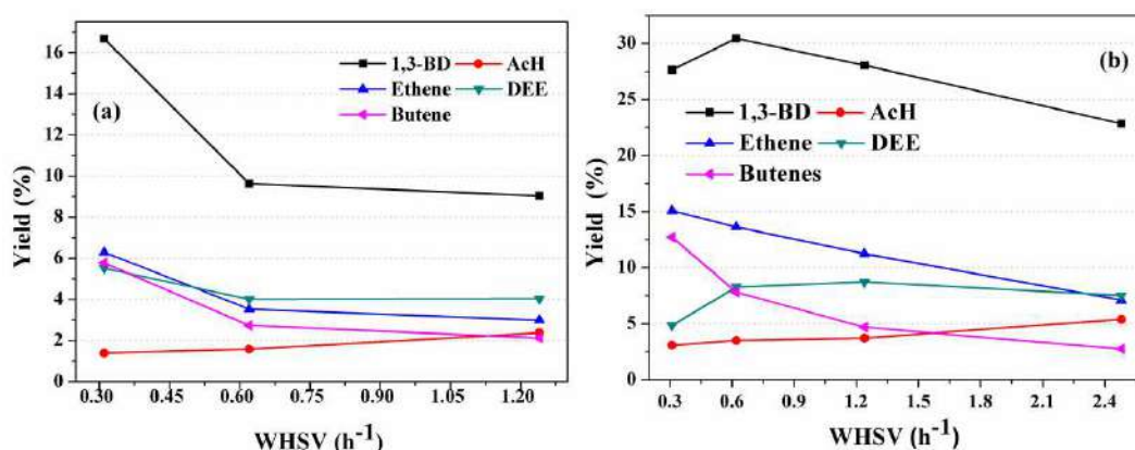
Figure 4.3.20 - Effect of WHSV on yields of the main carbon containing products at (a) 325 °C and (b) 375 °C. (ZrZn/MgO-SiO 2 -(50:50), TOS of 3 h).
