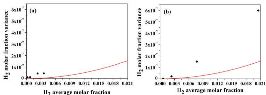
Figure 4.2.10 – Variances of hydrogen molar fractions for catalytic reactions (●) and chromatographic measurement fluctuation model (-) as functions of hydrogen average molar fractions for catalysts MgO-SiO 2 -(50:50) (a) and MgO-SiO 2 -(95:5) (b).
