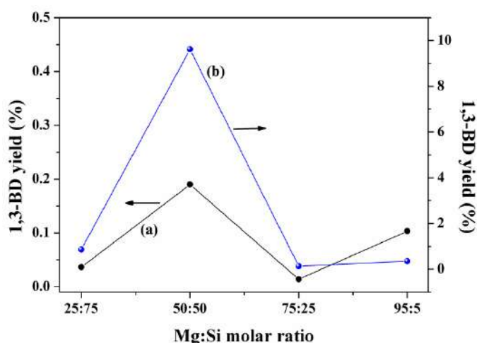
Figure 4.3.2 Mg:Si molar ratio effect on 1,3-BD yield (a) MgO-SiO 2 systems and (b) MgO-SiO 2 systems containing ZrO 2 and ZnO (T of 325 °C, TOS of 3 h, WHSV of 0.62 h -1 , contact time of 4 s).
