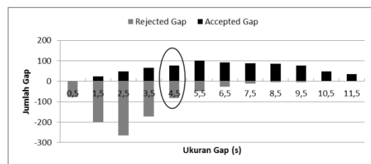
Gambar 4 Penentuan gap kritis metode Greenshields
