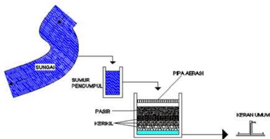
Gambar 4. SIPAS Saringan Pasir Lambat
