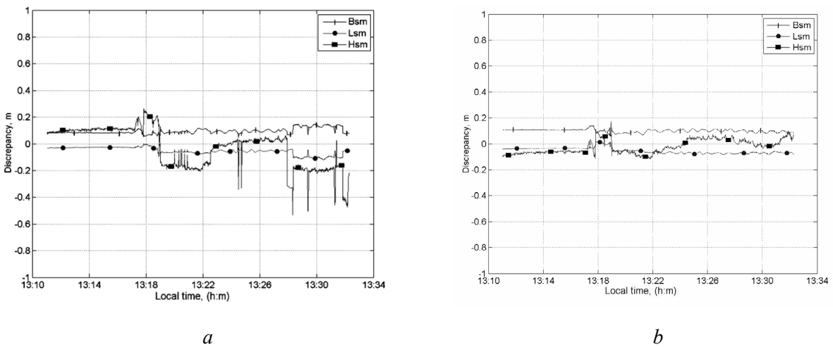
Fig. 9. Discrepancies of «leveling»-algorithm solution ( a ), modified algorithm solution ( b ) and reference coordinates in local system of coordinates (plane coordinates B, L and height H)
