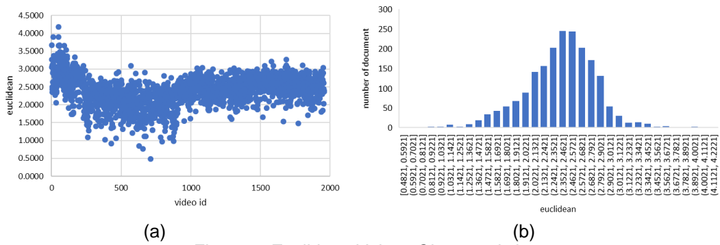
Figure 8. Euclidean Values Characteristic
