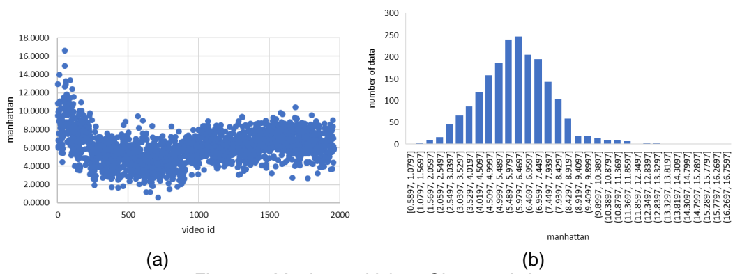
Figure 9. Manhattan Values Characteristic
