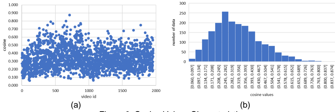
Figure 6. Cosine Values Characteristic
