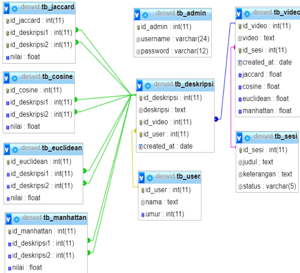
Figure 2. Physical Data Model
