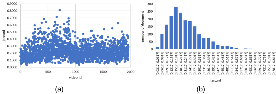
Figure 7. Jaccard Values Characteristic
