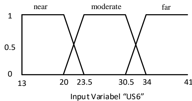
Figure 9. The Membership Functions of US6 Sensor
