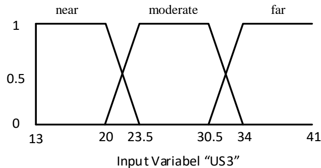
Figure 6. The Membership Functions of US3 Sensor
