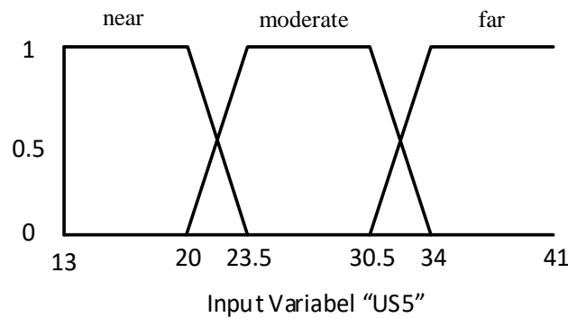
Figure 8. The Membership Functions of US5 Sensor
