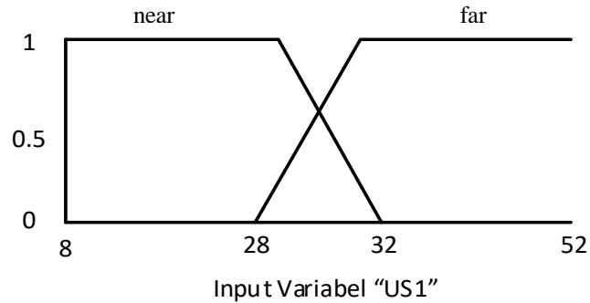
Figure 4. The Membership Functions of US1 Sensor
