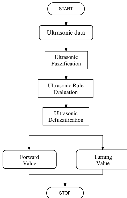
Figure 2. Fuzzy Logic Process in Robot
