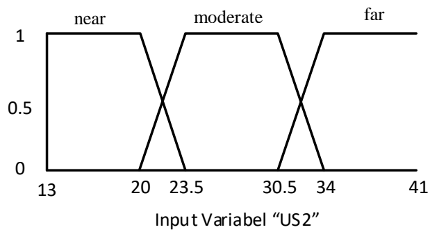
Figure 5. The Membership Functions of US2 Sensor
