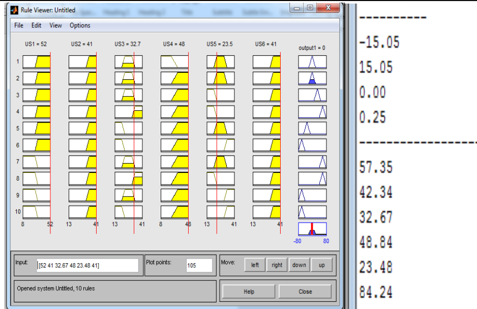
Figure 11. Display of Rule Viewer and Serial Monitor
