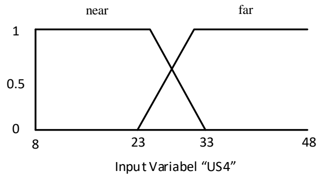
Figure 7. The Membership Functions of US4 Sensor
