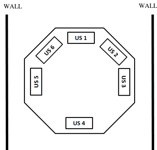
Figure 3. The Configuration of Ultrasonic Sensor Locations
