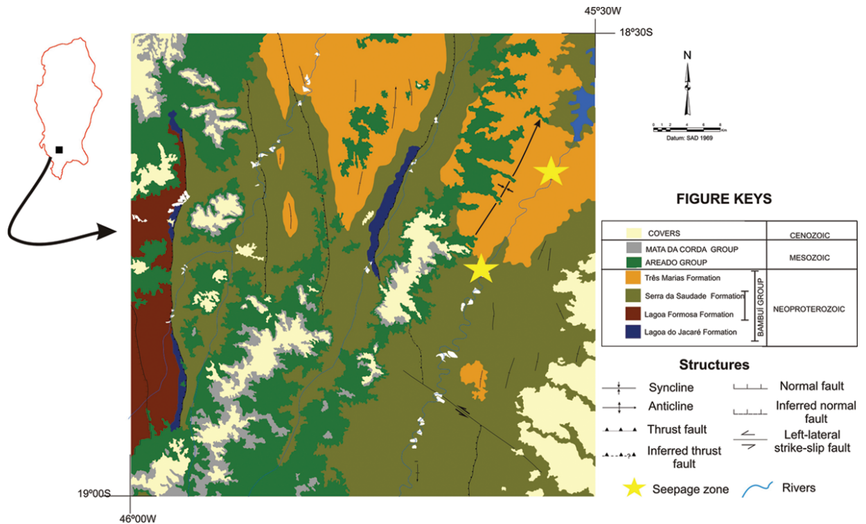
Figure 2 – Simplified geological map of Serra Selada Quadrangle (1:100.000), modified after Reis (2010).
