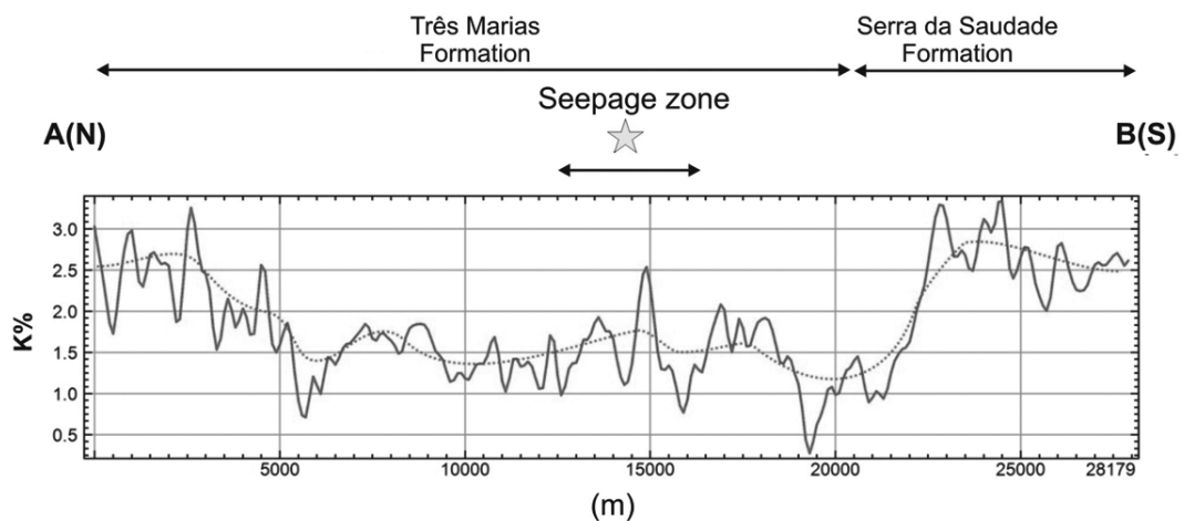
Figure 10 – Potassium contents (K%) along a section (A-B) N-S oriented that intersects the seepage zone of Northeastern Serra Selada Quadrangle. The potassium contents were obtained from the Gamma-ray spectrometry Map – K channel, presented in Figure 9. Locations of the emanation zones and respective sections are in Figures 2 and 9, respectively.
