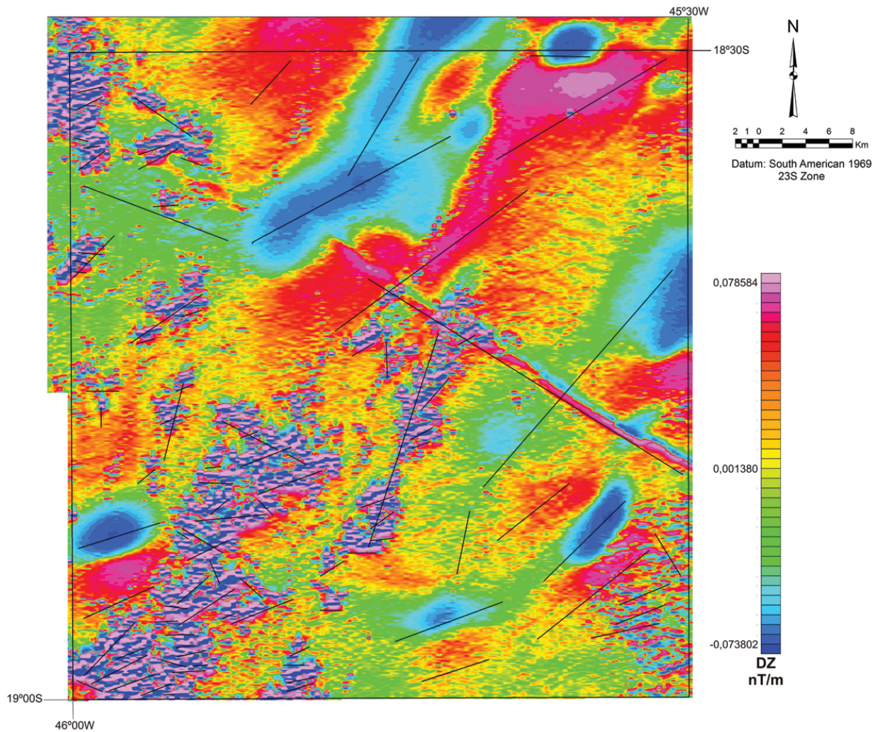
Figure 6 – First Vertical Derivative of the Anomalous Field Map, Serra Selada Quadrangle (1:100.000). The black traces correspond to interpreted magnetic lineaments.
