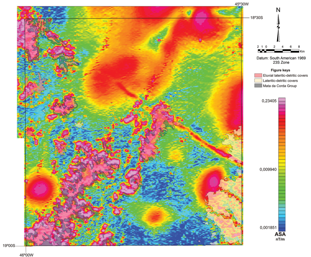
Figure 8 – Superimposition of the Analytical Signal Amplitude Map and the main outcropping magnetic units (compiled from field data), Serra Selada Quadrangle (1:100.000).
