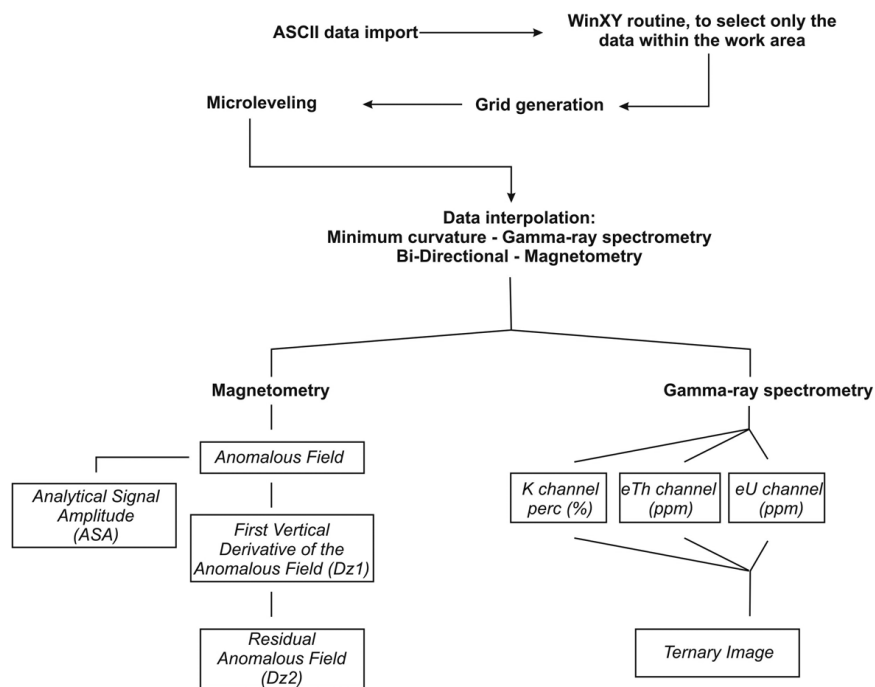
Figure 4 – Flowchart of the aeromagneto and aerogamma-ray spectrometry data processing in the creation of geophysical maps of Serra Selada Quadrangle (1:100.000).
