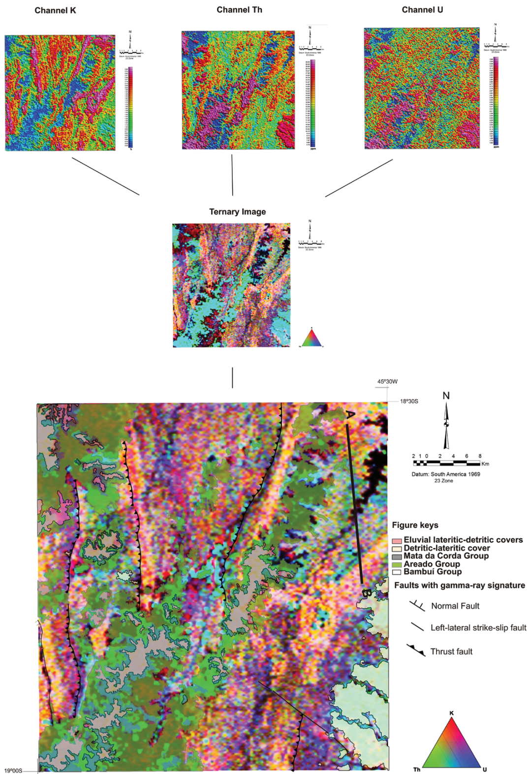
Figure 9 – Aerogamma-ray spectrometry in K, Th and U channels in Serra Selada Quadrangle area (1:100.000). The traces of the main mapped faults and lithostratigraphic units (Bambuí, Areado and Mata da Corda groups) were placed over the ternary image. Expressive potassium highs, locally, set the limits of the verdete bodies that mainly occur in the southeast portion of the quadrangle.
