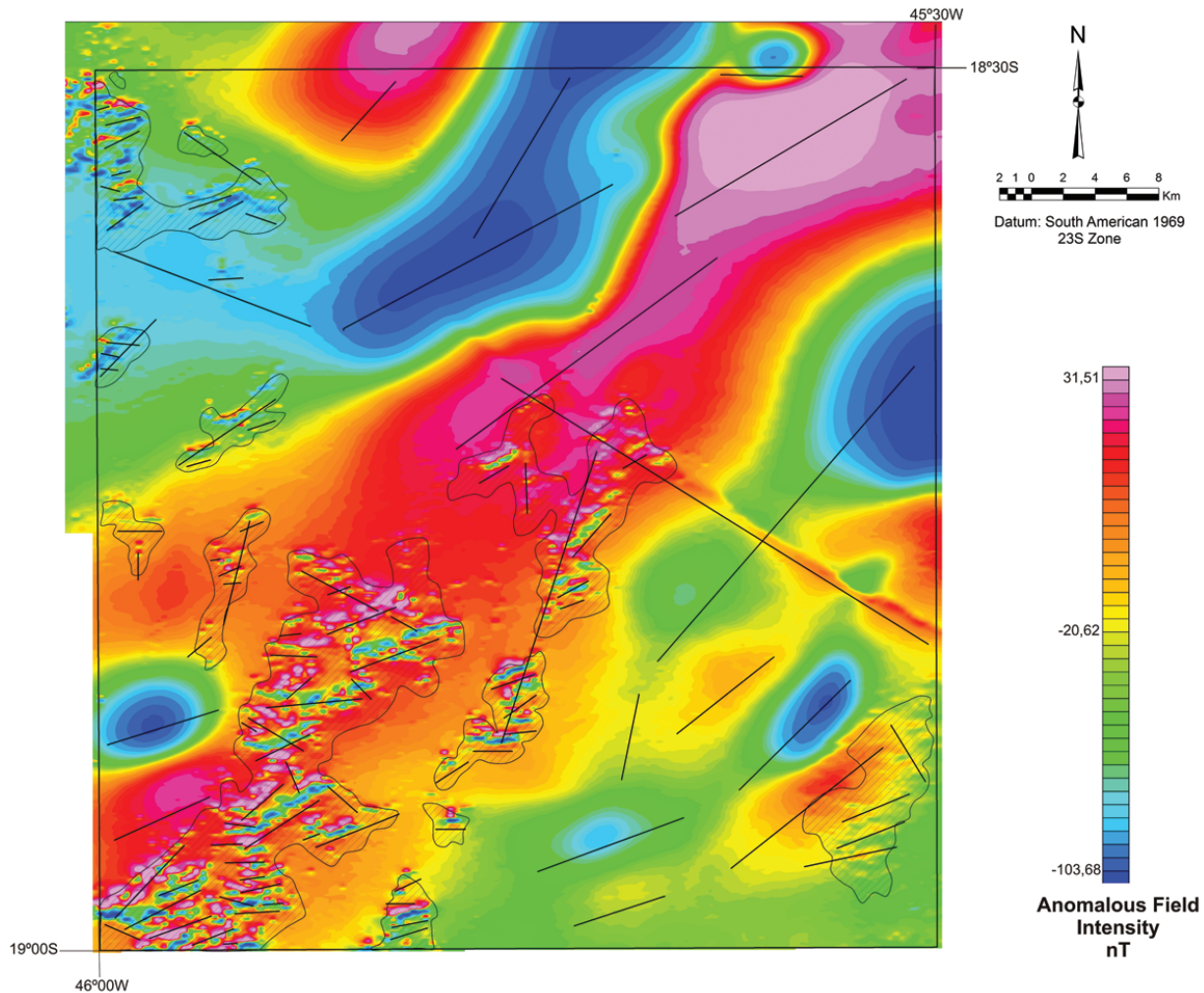
Figure 5 – Anomalous Magnetic Field Map (IGRF removed) of Serra Selada Quadrangle (1:100.000). The hachured areas correspond to high frequency anomalies; the other areas correspond to domains of low frequency anomalies (magnetometric background). The black traces correspond to interpreted magnetic lineaments.
