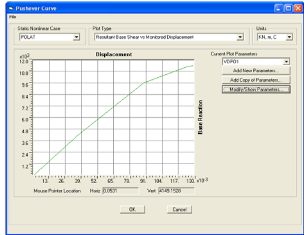
(b) Pushover curve for the direction-Y
