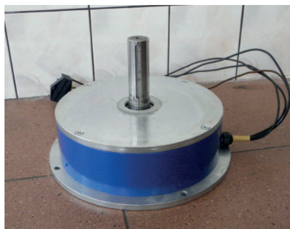
Gambar 3. Generator VAWT 500 watt.
