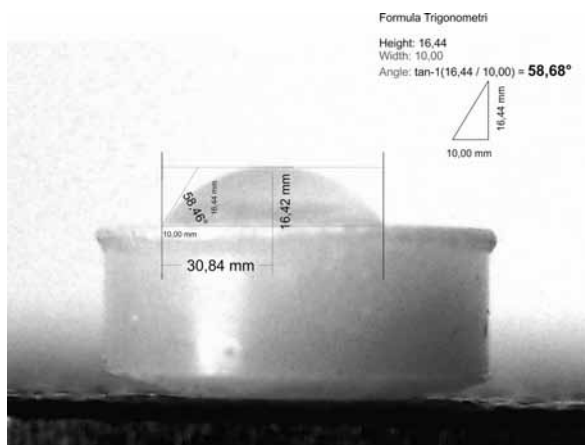
Figure 3 Application of Trigonometry Formula to Calculate the Contact Angle
