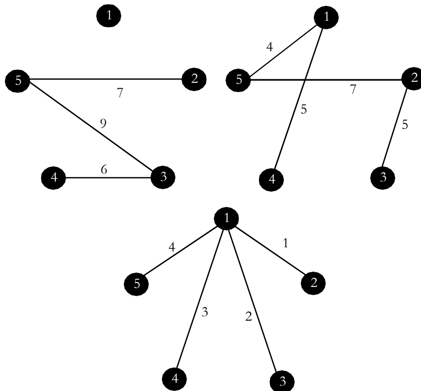
Figure 3. In a clockwise manner from the left above, a tree in G , a Spanning Tree in G , a Minimum Spanning Tree G
