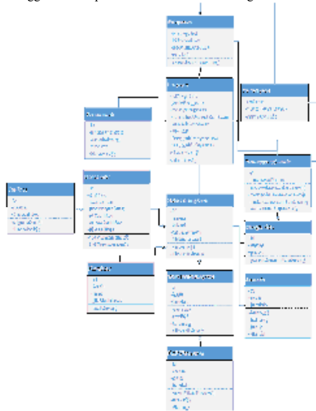
Gambar. 4 Class diagram
