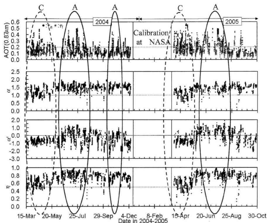
Fig.1 Radiometry of aerosols at Higashi-Osaka site from 15 March 2004 to 30 October 2005, where AOT ( \tau_\lambda , \tau_f ) at a wavelength of 0.87\mu\text{m} , Ångström exponent \alpha , its second derivative \alpha' and the optical fraction of fine-mode particles \eta are presented. Refer to the text in section 2 with respect to clusters (A) and (C).
