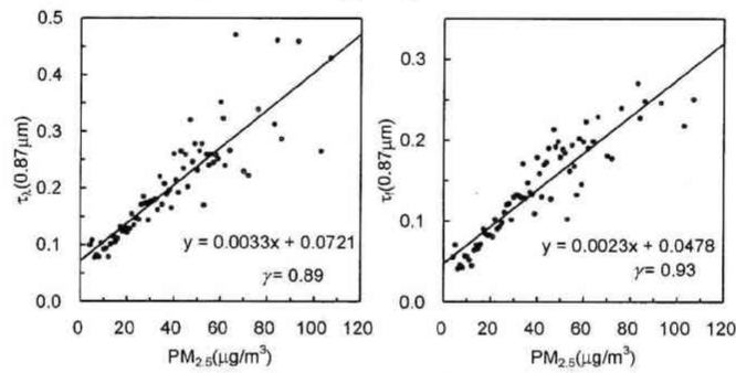
Fig.4 Scattergrams of PM 2.5 against AOT (0.87µm) as total aerosol optical thickness ( \tau_\lambda ) (left) and fine mode-optical thickness ( \tau_f ) (right).
