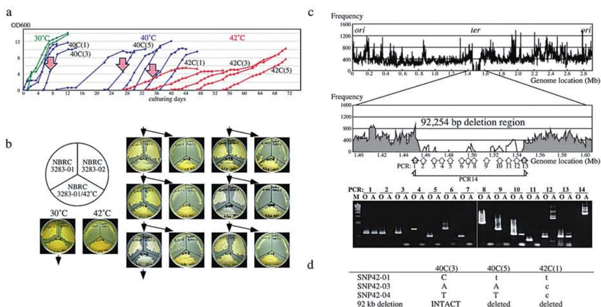
Fig 6. Adaptation to an unviable environment at high-temperatures.
