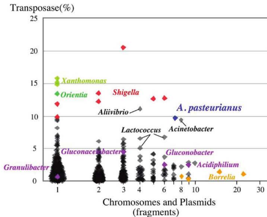
Fig 4. Features of A. pasteurianus hyper-mutability.
