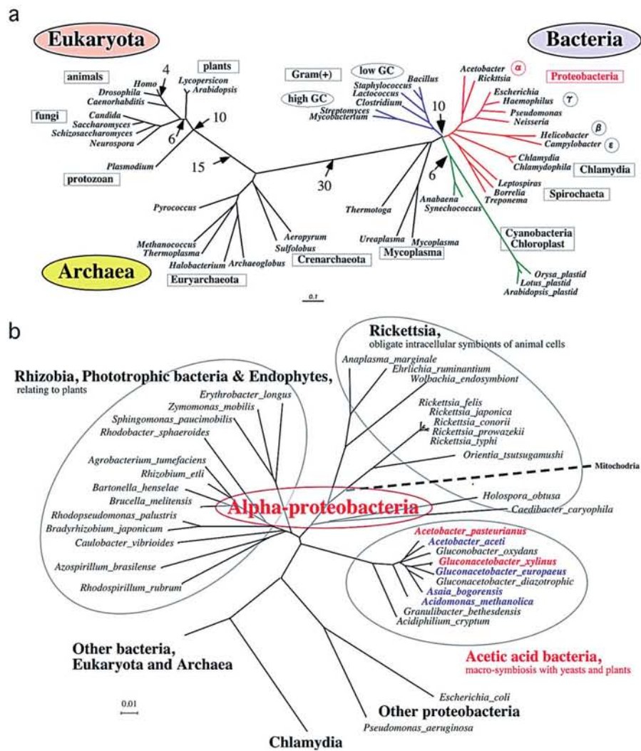
Phylogenetic tree of life and acetic acid bacteria based on small ribosomal RNA sequences
