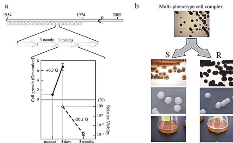
Fig 1. Mutation accumulation within maintenance of A. pasteurianus IFO 3283 for 21 years.
