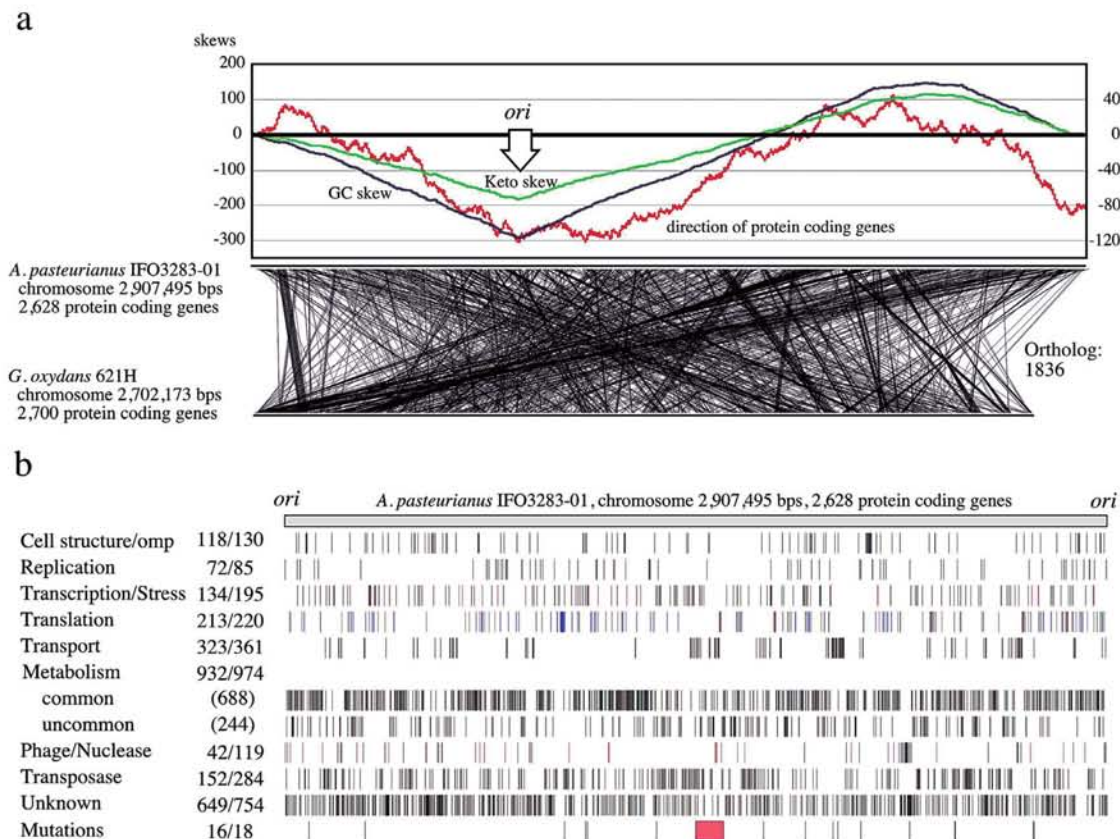
Fig 2. Genome map and structure of A. pasteurianus IFO 3283-01 chromosome
