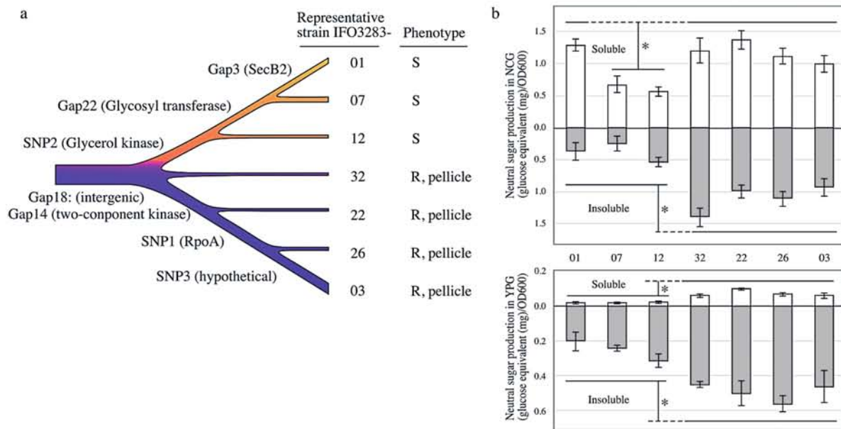
Fig 3. Mutation accumulation within maintenance of A. pasteurianus IFO 3283 for 21 years.
