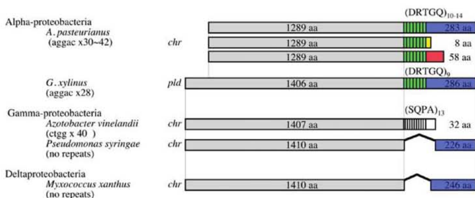
Fig 5. A schematic illustration of the structures of gene products with hyper-mutable tandem repeat sequences.
