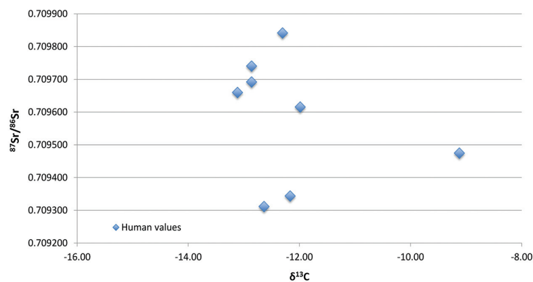
Fig. 7. Scatterplot ^{87}Sr/^{86}Sr vs. \delta^{13}C .
