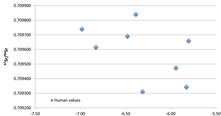
Fig. 8. Scatterplot ^{87}\text{Sr}/^{86}\text{Sr} vs. \delta^{18}\text{O} .
