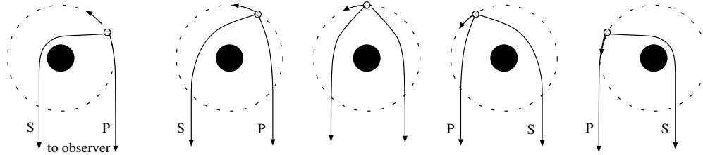
Figure 6. Prograde and retrograde photon trajectories. The pulsar is shown orbiting in the counterclockwise direction around a much more massive black hole. The leftmost cartoon shows that the observing radio telescope receives a primary (P) direct pulse and a highly bent secondary (S) pulse. The subsequent panels show trajectories as the pulsar continues its orbital motion. The primary trajectory has increased bending and the secondary less, until the pulsar is directly opposite the receiver and the two trajectories are symmetric. The following panels show how the prograde trajectory then becomes the primary (less bent) trajectory.
