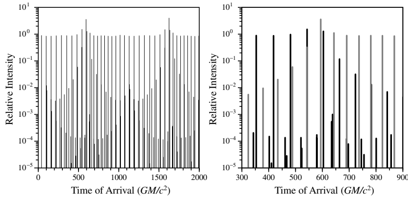
Figure 7. Relative intensity of pulses for the system shown in Figure 5.
