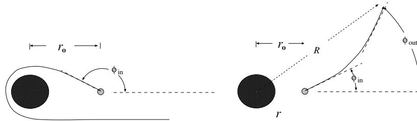
Figure 1. Photon path from the radial coordinate r_0 to R . The path on the right indicates mild bending of the path due to spacetime curvature. On the left is shown the highly bent photon path which has an impact parameter near the critical value of photon capture, and a \phi_{\text{out}} , at large R , of 2\pi .
