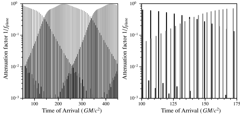
Figure 8. Same plot as in Figure 5, but for a more relativistic system, with orbital radius 10 \times GM/c^2 , and with rotation rate 47 times the orbital frequency.
