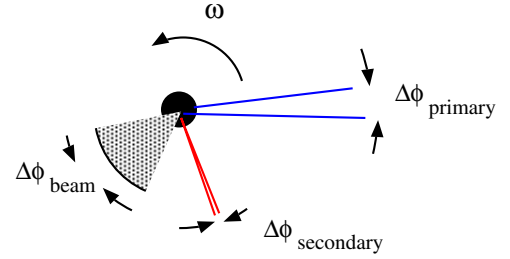
Figure 4. Pulsar beam sweeping through the narrow range of directions that connect to the receiver.
