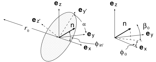
Figure 3. Triads and angles used to define photon directions.
