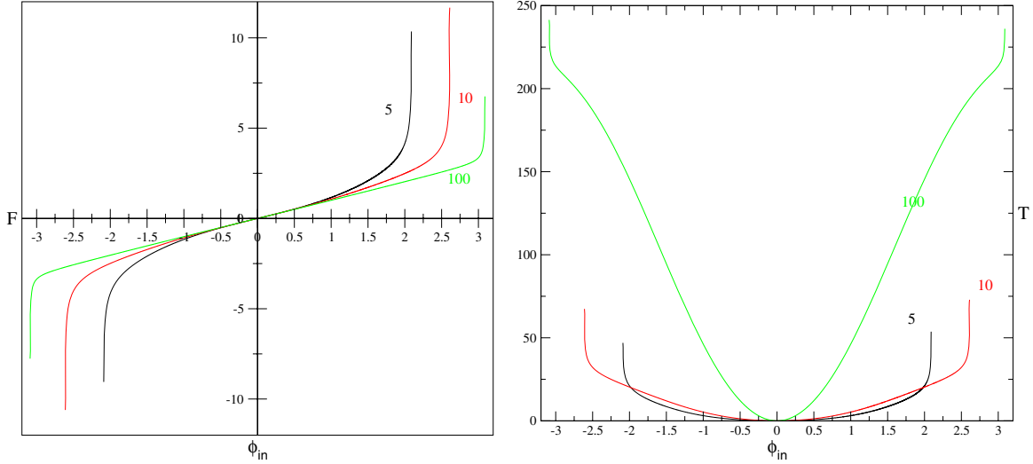
Figure 2. Universal functions F and T . Curves are labeled with the values of r_0/M : 5, 10, and 100. The values of \phi_{\text{crit}} , from Equation (4) are, respectively, 2.0895, 2.6109, and 3.0896.
