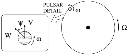
Figure 10. Orbital motion of the pulsar at frequency \Omega , the parallel transported spatial direction V^\mu , and the pulsar beam direction W^\mu rotating at frequency \omega relative to V^\mu , as observed in a frame comoving with the pulsar.
