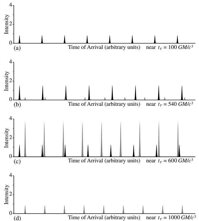
Figure 9. Appearance of received radio pulses for several orbital epochs of a pulsar orbiting with radius 30 \times GM/c^2 . The pulsar rotation rate is assumed to be much greater than the orbital frequency.
