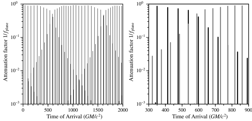
Figure 5. Factor 1/f_{\text{plane}} for photon capture events from a pulsar with orbital radius 30 \times GM/c^2 , and the pulsar rotation rate 20.2 times the orbital rotation rate. Events for several orbits are shown on the left. Details are shown on the right for the orbital epoch during which the pulsar is on the far side of the hole.
