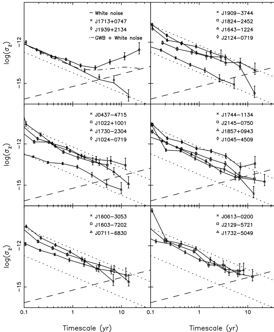
Figure 2. \sigma_z stability parameter for the 20 pulsars in our sample. The dotted slanted lines represent white noise levels of 100 ns (bottom line) and 10 \mu s (top line); the dashed slanted line shows the steepness introduced to pre-fit residuals by a hypothetical GWB (see Section 1); pulsars whose curve is steeper than this line (like PSR J1939+2134) can therefore be expected to be of little use to PTA efforts on long time-scales. The top-left figure further shows the average \sigma_z values resulting from 1000 simulations of white noise sampled at the times of the PSR J1713+0747 data set and fitted for the PSR J1713+0747 timing model parameters (full line). This demonstrates that the PSR J1713+0747 data do not – within the sensitivity provided by the \sigma_z statistic – contain a significant, steep red-noise process. The dash-dotted line in the top-left figure shows the average of 2000 simulations for white noise combined with a GWB, sampled at the times of the PSR J1939+2134 data set and fitted for pulse period and period derivative. These simulated results provide an example of the combined effect sampling and model fitting can have on the \sigma_z statistic, even in the case of white noise.
