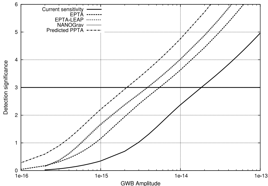
Figure 4. Sensitivity curves for different PTA efforts. Note the ‘NANOGrav’ and ‘EPTA–LEAP’ curves are practically coincident. Gravitational waves are predicted to exist in the range 10^{-15} – 10^{-14} (see text and Table 7 for more information).
