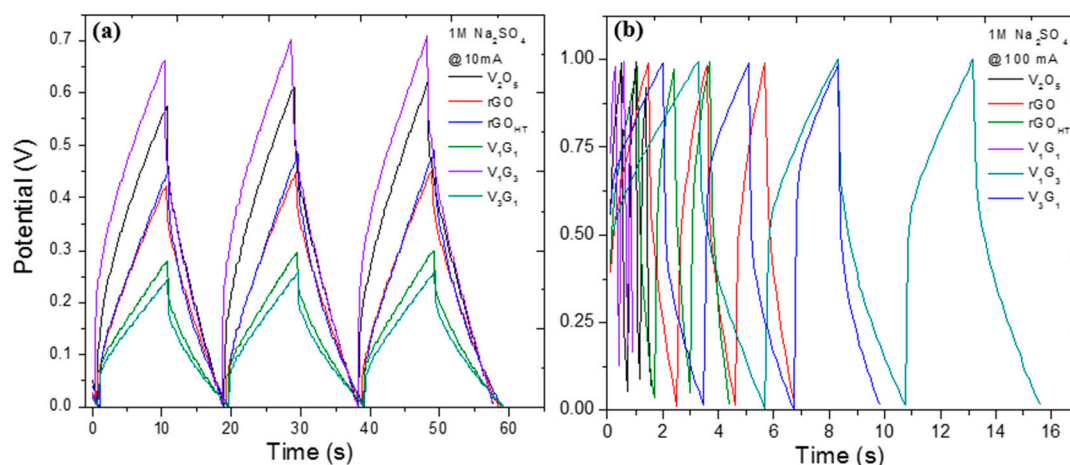
Figure 5. Galvanostatic charging-discharging profiles between 0.01 and 1.0 V at current densities of (a) 1 and (b) 10 \text{A} \cdot \text{g}^{-1} showing characteristics discharging capacitor shapes.
