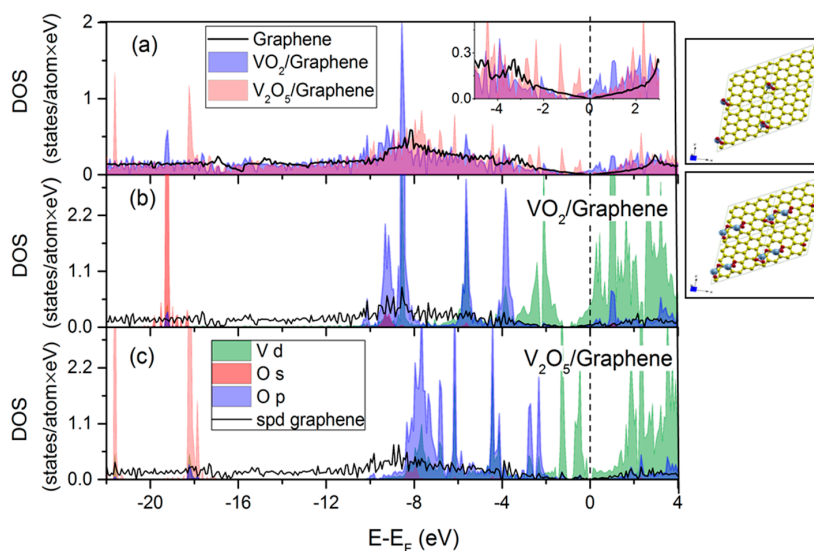
Figure 9. Density functional theory (DFT) calculations. Total electronic density of state (DOS) spectra per atom eV for (a) clean graphene, \text{VO}_2/\text{graphene} , \text{V}_2\text{O}_5/\text{graphene} ( 4 \times 4 graphene supercell); partial DOS spectra of (b) \text{VO}_2/\text{graphene} and (c) \text{V}_2\text{O}_5/\text{graphene} for V d, O 2s and O 2p orbitals and spd graphene. Schematics of graphene, vanadium oxide and vanadium pentoxide clusters on the 4 \times 4 graphene supercell (top view, right panel). The vertical line is the Fermi level.
