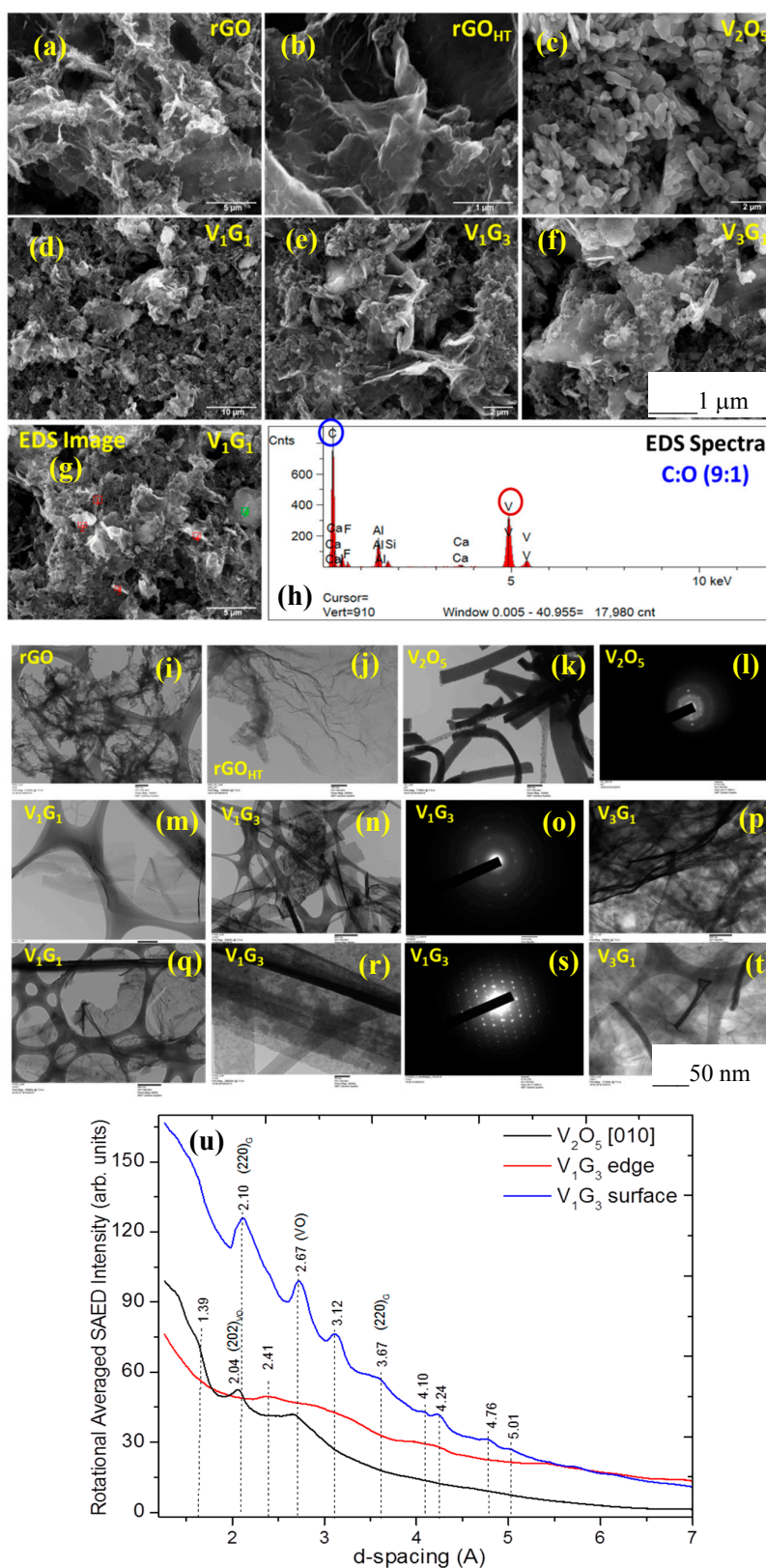
Figure 2. (a–g) SEM micrographs; (h) EDS spectra; TEM micrographs of (i) rGO; (j) rGO HT ; (k) V 2 O 5 ; (m,q) V 1 G 1 ; (n,r) V 1 G 3 ; (p,t) V 3 G 1 ; (l,o,s) SAED and (u) the real space ( d_{hkl} ) intensity pattern revealing the crystal structure of ‘hybrids’ for the representative samples studied. The surface morphology and semicrystalline nature of VNBs with rGO HT nanosheets is apparent (scale bars are shown at the bottom of the images).
