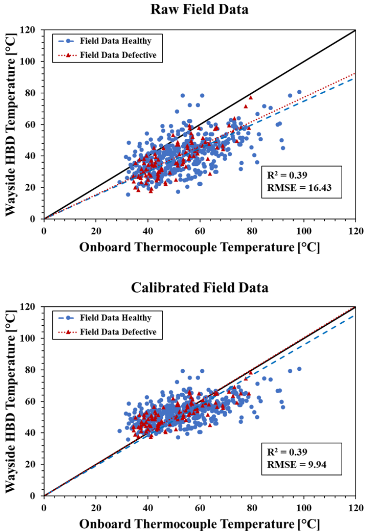
Figure 11. Raw (top plot) and calibrated (bottom plot) field-test wayside HBD temperature versus onboard thermocouple temperature.
