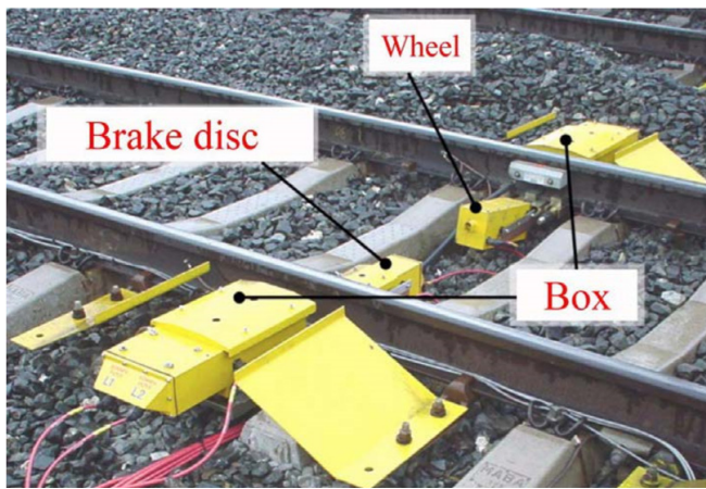
Figure 1 . Photograph of a wayside hot-box detector system [3].
