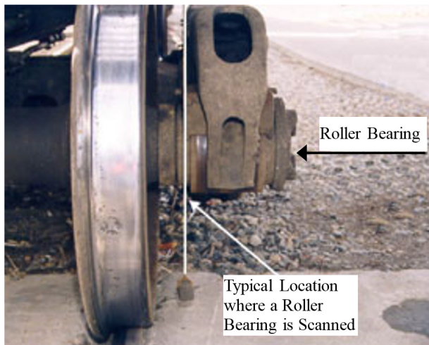
Figure 2 . Typical infrared sensor scanning location for field wayside hot-box detectors (HBDs) [4].
