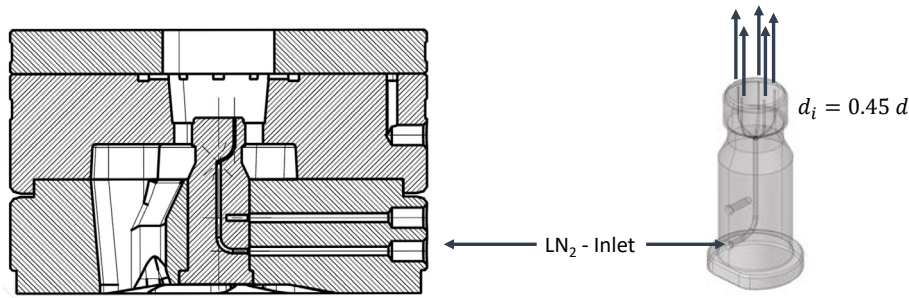
Figure 3: Cooling channel position and geometry for a five-chamber porthole die
