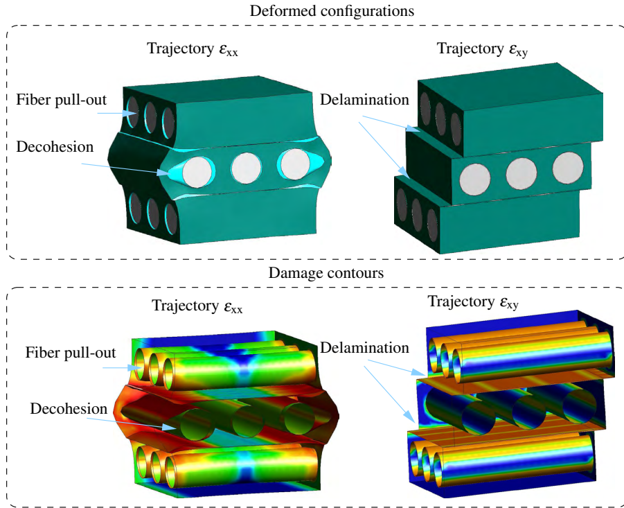
Figure 3: Deformed configuration and damage contours at trajectories \varepsilon_{xx} (left) and \varepsilon_{xy} (right).
