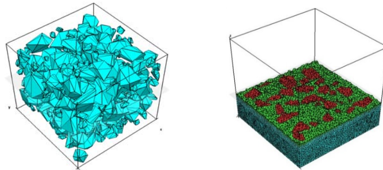
(a) A full 3D mesoscale model: meso-geometry
