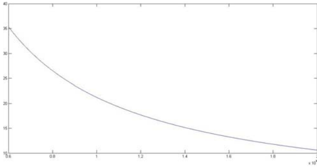
Figure 4. Variation of the frequency for a minimum 10 Hz frequency value for a variation of the potentiometer between 6.0 kΩ and 20 kΩ using MatLab®.
