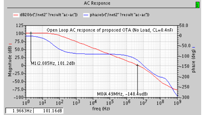
Fig. 7.- AC-Response of the proposed OTA, with C_L=0.4 nF , R_L=\infty .
