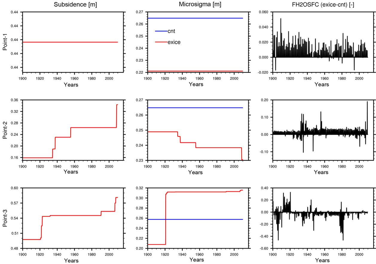
Figure 5. Time series of subsidence, \sigma_{micro} , and f_{h2osfc} variables from the Exice and Control experiments at three selected sites. Point 1: 54° N, 272° E; Point 2: 64° N, 80° E; Point 3: 65° N, 70° E.
