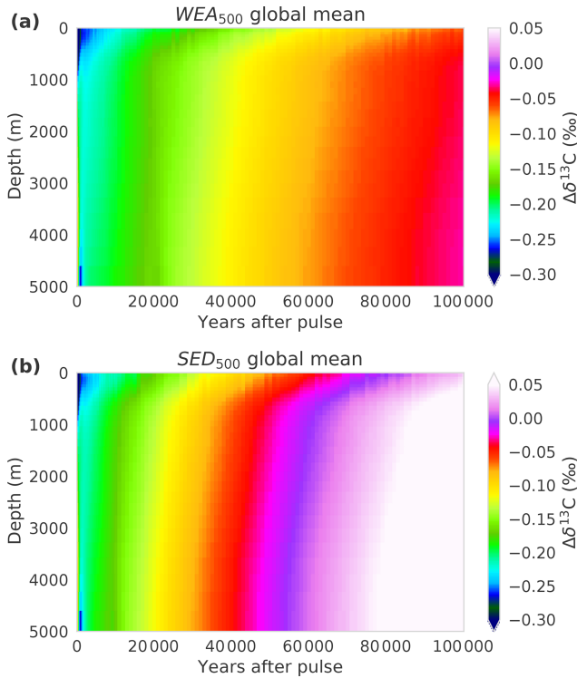
Figure A1. Hovmöller-type diagram showing the temporal evolution of the global-mean vertical profile of \Delta\delta^{13}\text{C}_{\text{DIC}} for experiments (a) \text{WEA}_{500} and (b) \text{SED}_{500} .
