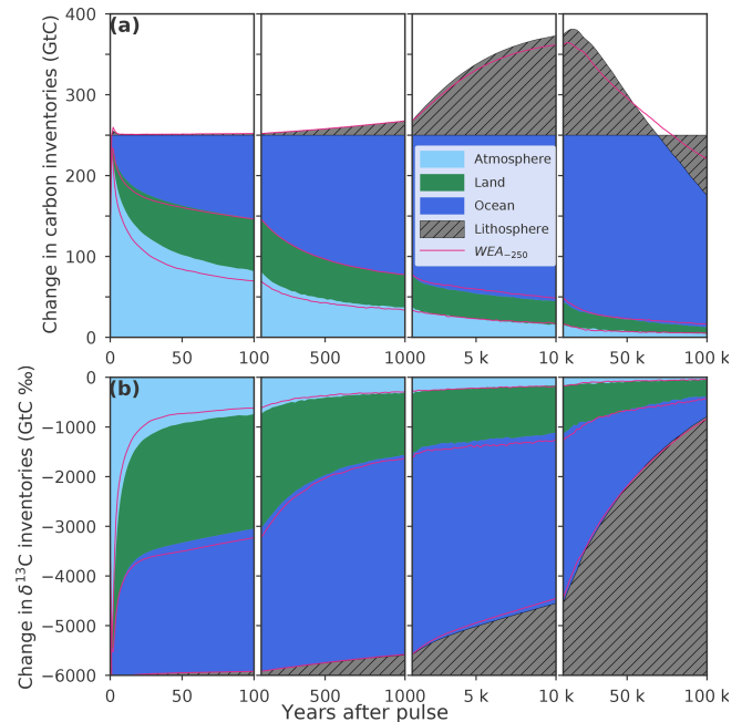
Figure 3. Inventories of the (a) carbon and (b) \delta^{13}\text{C} perturbations for experiment WEA 250 . Shown are inventories of the perturbations in the atmosphere (light blue), the land biosphere (green), and the ocean (blue). Hatching indicates the influence of changes in the lithosphere (including sediments) due to CaCO 3 compensation and imbalances in the weathering and burial fluxes on the carbon and isotopic inventories of the ocean–atmosphere–land system. For carbon, this inventory is elevated above the pulse perturbation of 250 GtC until about 70 kyr and depleted thereafter. For \delta^{13}\text{C} , the atmosphere–ocean–land inventory is continuously reduced over the course of the simulation. Magenta lines show results for experiment WEA -250 multiplied by -1 .
