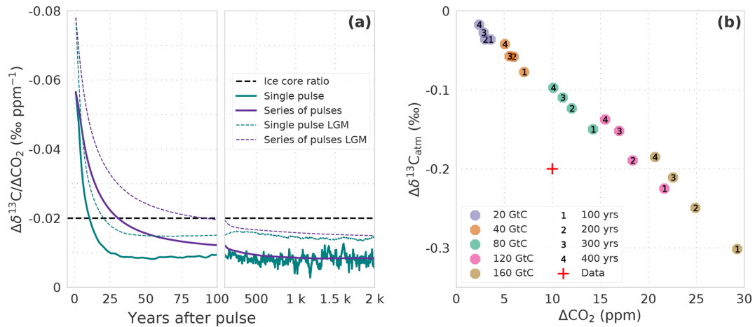
Figure 8. (a) Temporal evolution of the ratio of \Delta\delta^{13}\text{C} to \Delta\text{CO}_2 in the atmosphere. Results are from simulations \text{WEA}_{100} forced by preindustrial boundary conditions (solid lines) and \text{LGM}_{100} forced by Last Glacial Maximum boundary conditions (thin dashed lines). Carbon is released as a single pulse at year 0 (green lines) or assumed to be released at a uniform rate from year 0 to the year plotted (purple lines; see main text). The dashed horizontal line indicates a \Delta\delta^{13}\text{C} -to- \Delta\text{CO}_2 ratio of -0.2\text{‰} to 10 ppm as seen in ice core records for HS1 and HS4. (b) Response in \Delta\text{CO}_2 and \Delta\delta^{13}\text{C}_{\text{atm}} to a uniform release of 20, 40, 80, 120, and 160 GtC of isotopically light carbon ( \delta^{13}\text{C} = -24\text{‰} ) to the atmosphere over 100, 200, 300, and 400 years (numbers). Shown is the mean over 30 years starting in the last year of the release. The red cross indicates the approx. \Delta\delta^{13}\text{C} -to- \Delta\text{CO}_2 change as seen in ice core records for HS1 and HS4 (Bauska et al., 2016, 2018).
