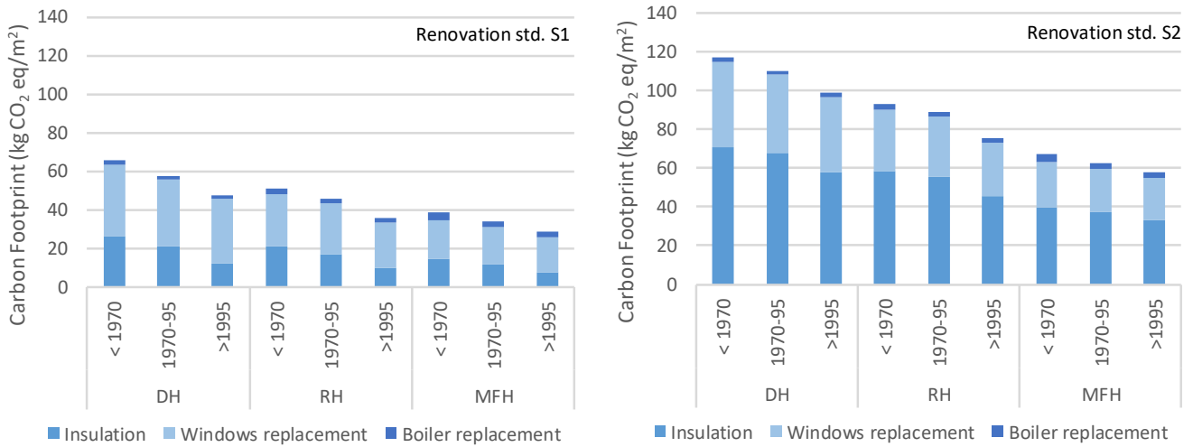
Figure 5 Average carbon footprint of renovation residential buildings in Esch-sur-Alzette per floor area unit per housing type (detached houses DH, row houses RH and multi-family houses MFH) and period of construction, implementing different renovation standards (S1 and S2).
