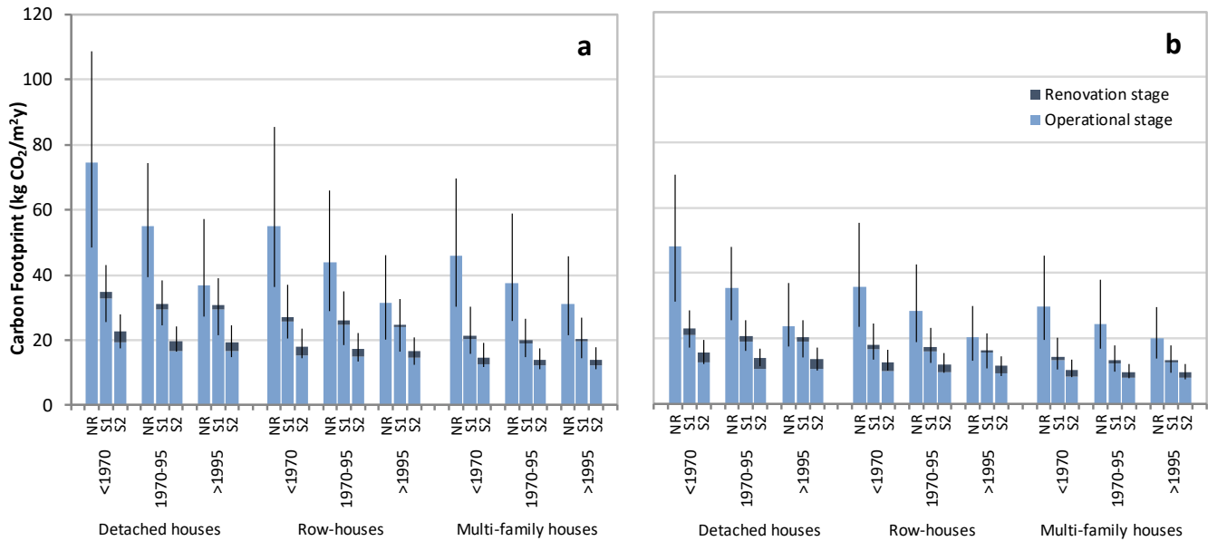
Figure 4 Carbon footprint along the residual life-cycle of residential buildings in Esch-sur-Alzette per floor area unit per housing type and period of construction without renovation (NR) and with different renovation standards (S1 and S2). Bars indicate median values; whiskers indicate 5% and 95% quantiles. Results are shown for calculation with fixed (a) and time-dependent (b) characterization factors.
