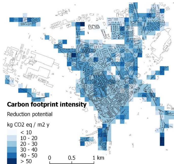
Figure 6 Spatial distribution of carbon footprint intensity reduction potential of residential buildings in Esch-sur-Alzette after implementing renovation measures (renovation standard S1) in kg CO 2 eq. per floor surface area per year.
