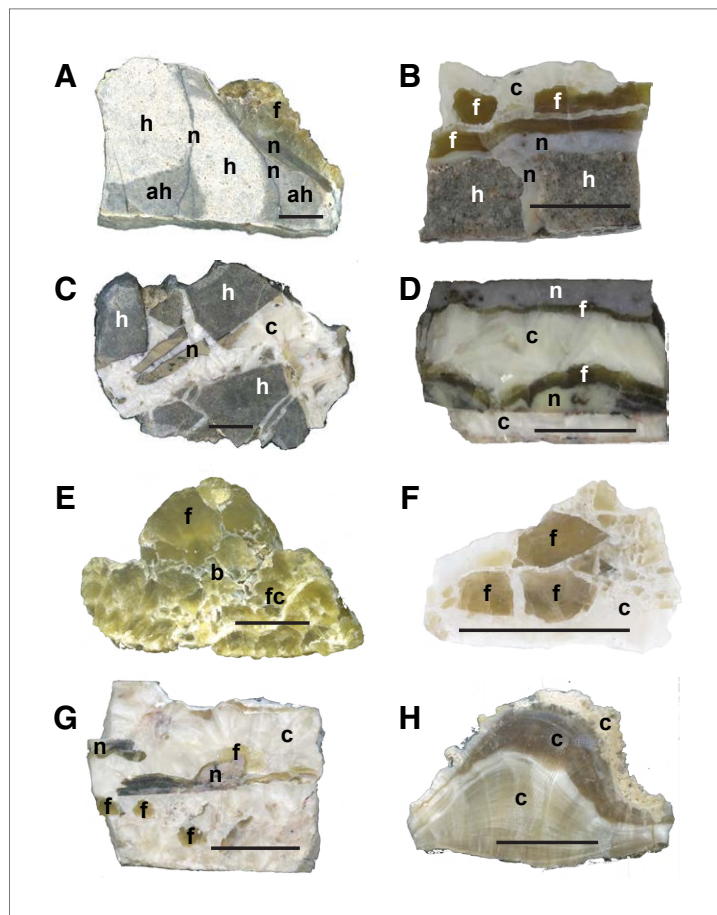
Figure 2. Visible light images of the samples from the fracture. (A) Host rock with small veins that are filled by fluorite and capped by fluorite. (B) Fractured host rhyolite with fluorite between fragments and on surfaces followed by fluorite, which is brecciated and cemented by calcite. (C) Brecciated host rhyolite and fluorite that is cemented by calcite. (D) Layered vein material with the calcite on the bottom appearing to be the surface upon which fluorite followed by fluorite followed by calcite grew. These minerals appear to come from the top and bottom. (E) Brecciated green fluorite with calcite filling between some fragments. (F) Brecciated fluorite with calcite cement. (G) Breccia with fluorite and calcite clasts. (H) Two generations of calcite. The white to amber calcite is highly enriched in rare-earth elements (REEs). The brown calcite is low in REE but has high U-Pb ratios. Labels are: h—host; ah—altered host; n—nacrite; f—fluorite; fc—fluorite with calcite; c—calcite; b—brecciated zone. Not visible here is the yttrium and heavy rare-earth element (YHREE) carbonate that lines the breccia clasts and occurs between fluorite and calcite. Scale bars are all 1 cm.
