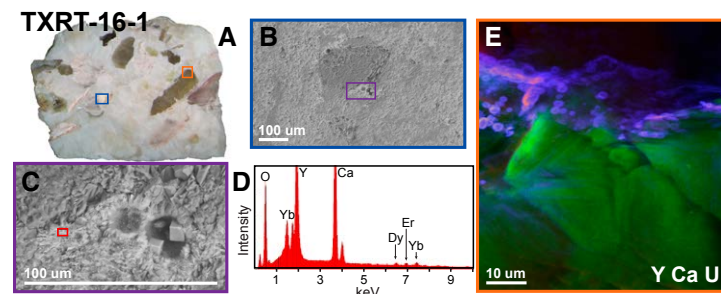
Figure 7. (A) Visible light image of vein breccia. (B) Scanning electron microscopy (SEM) image of area in blue box on A. (C) SEM image of area in purple box on B; shows nodules of yttrium and heavy rare-earth element (YHREE) mineral. (D) Energy-dispersive X-ray (EDX) spectra from area outlined by red box in C. (E) Synchrotron X-ray fluorescence (S-XRF) elemental image taken at 13-ID-E beamline of the edge of a fluorite clast; area of image outlined by orange box in A. RGB coloration is Y, Ca, and U, respectively.
