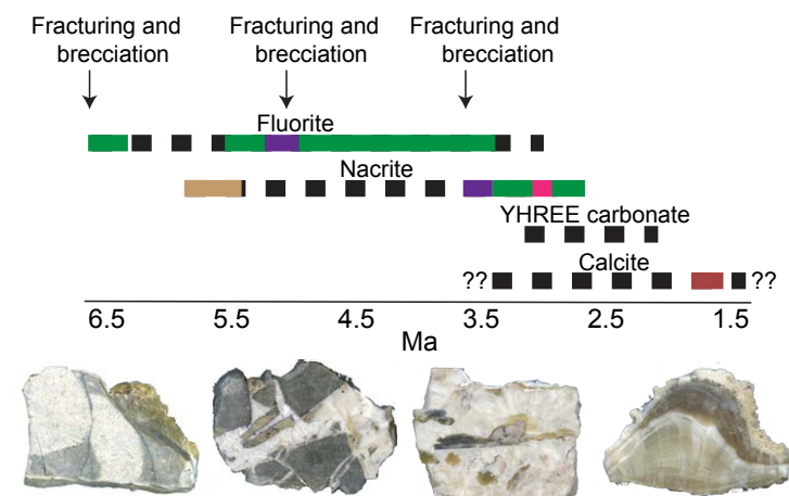
Figure 14. Paragenesis determined by the ages of fluorite, nacrite, and calcite. Each labeled line represents timing of crystallization of the specified mineral. Line colors represent mineralization color (i.e., purple = purple fluorite or purple nacrite crystallization). Dotted lines indicate undated (but possible) mineralization. Sample photos are representative of mineralization from 6.5 Ma to 1.5 Ma (going from left to right, decreasing in age). YHREE—yttrium heavy rare-earth element.
