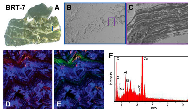
Figure 9. (A) Visible light image of brecciated green fluorite sample as shown in Figure 3E. (B) Scanning electron microscopy (SEM) image from inset area outlined in blue box in A. (C) SEM image of area outlined in purple box in B. (D) X15B RGB map of Y, Si, U, respectively. (E) X15B RGB map of Y, S, and U, respectively. (F) Energy-dispersive X-ray (EDX) spectra of calcite show that Al and Si are present even at high magnification.
