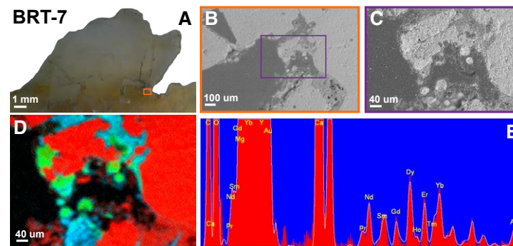
Figure 5. (A) Visible light image of brecciated green fluorite. (B) Scanning electron microscopy (SEM) image from the orange boxed area in A. (C) Further zoom on the brecciated fluorite; area indicated by the purple box in B. (D) RGB color image of area in C; red—Ca (fluorite); blue—Mg (dickite and nacrite); green—Y (YHREE-bearing carbonate). (E) Energy-dispersive X-ray (EDX) spectra of yttrium and heavy rare-earth element (YHREE) carbonate mineral. Note resorbed texture in the fluorite and the close spatial association of the YHREE mineral and dickite.
