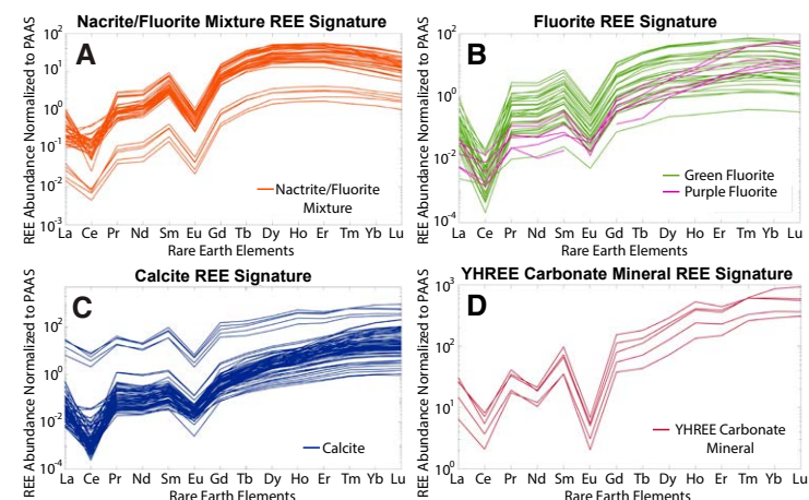
Figure 11. (A) Rare-earth element (REE) pattern for nacrite and fluorite mixture; (B) REE pattern for green and purple fluorite; (C) REE pattern for calcite; and (D) REE pattern for yttrium and heavy rare-earth element (YHREE) carbonate mineral.
