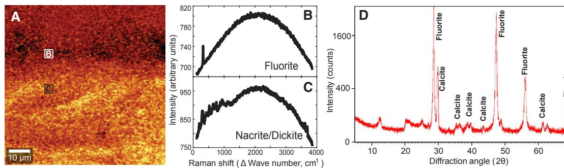
Figure 3. (A) Raman map of vein material. Dark region on top is fluorite (spectra shown in B); lighter region on the bottom is nacrite (spectra shown in C). (B) Raman spectra indicate fluorite. (C) Raman spectra from cryptocrystalline phase show the presence of nacrite. (D) X-ray diffraction (XRD) spectra of a selected cryptocrystalline phase indicate mixture of fluorite, calcite, and a weakly crystalline phase(s) consistent with nacrite.
