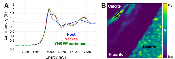
Figure 4. (A) Yttrium K-edge X-ray absorption near edge structure (XANES) (YHREE carbonate mineral—green; nacrite—red; host rock—blue). Data from submicron-resolution X-ray spectroscopy (SRX) at the National Synchrotron Light Source (NSLS) II. (B) Synchrotron X-ray fluorescence (S-XRF) map (blue—low concentration; yellow—high concentration) showing Y-rich mineral lining fluorite (rare-earth element) and Y-rich spots in the nacrite. Map dimensions are 0.2 × 0.2 mm. YHREE—yttrium heavy rare-earth element.
