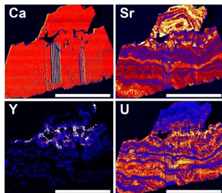
Figure 6. Synchrotron X-ray fluorescence (S-XRF) maps from X26A, National Synchrotron Light Source (NSLS). White bar is 1 cm. Lines and spots on surface are from laser ablation. Ca—calcium; Sr—strontium; Y—yttrium; and U—uranium.
