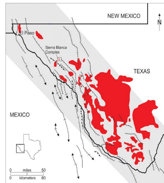
Figure 1. Location of the Sierra Blanca Complex (shown in red) relative to major geologic structures within the Trans-Pecos magmatic province. The gray shaded region represents the Texas lineament zone—a broad, ~80-km-wide zone of parallel transtensional faulting. Northwest-trending normal faults are related to Rio Grande rifting. Map modified from Muehlberger (1980), Price et al. (1990), and O'Neill et al. (2017).
