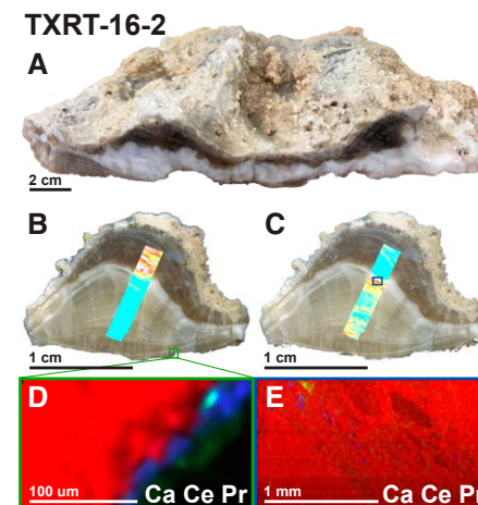
Figure 8. (A) Visible light photo of vein as shown in Figure 2H. (B) Cross section of slab cut from sample in A. Laser ablation map of U concentration (hot colors = high; cold colors = low). (C) Cross section of slab cut from sample in A. Laser ablation map of yttrium (Y) concentration (hot colors = high; low colors = low). (D, E) Composite RGB X-ray fluorescence (XRF) elemental maps taken at sub-micron-resolution X-ray spectroscopy (SRX); area corresponding to green and purple boxes in B and C, respectively. RGB maps are Ca, Ce, and Pr, respectively.
