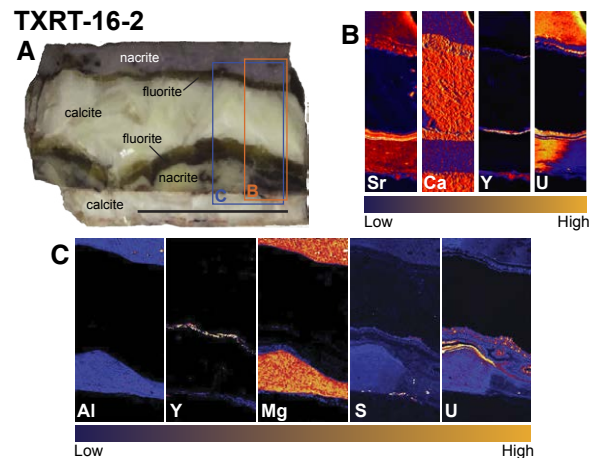
Figure 10. (A) Visible light image of a layered vein as shown in Figure 3D. Scale bar is 1 cm. (B) X-ray fluorescence (XRF) elemental maps of the Sr K-edge, Ca K-edge, Y K-edge, and U L-edge taken at X-ray fluorescence microprobe (XFM) beamline; area corresponding to the small orange rectangle in A. (C) XRF elemental maps of the Al K-edge, Y L-edge, Mg K-edge, S K-edge, and U M-edge taken at Tender Energy Spectroscopy (TES) beamline; area corresponding to the larger purple rectangle in A.
